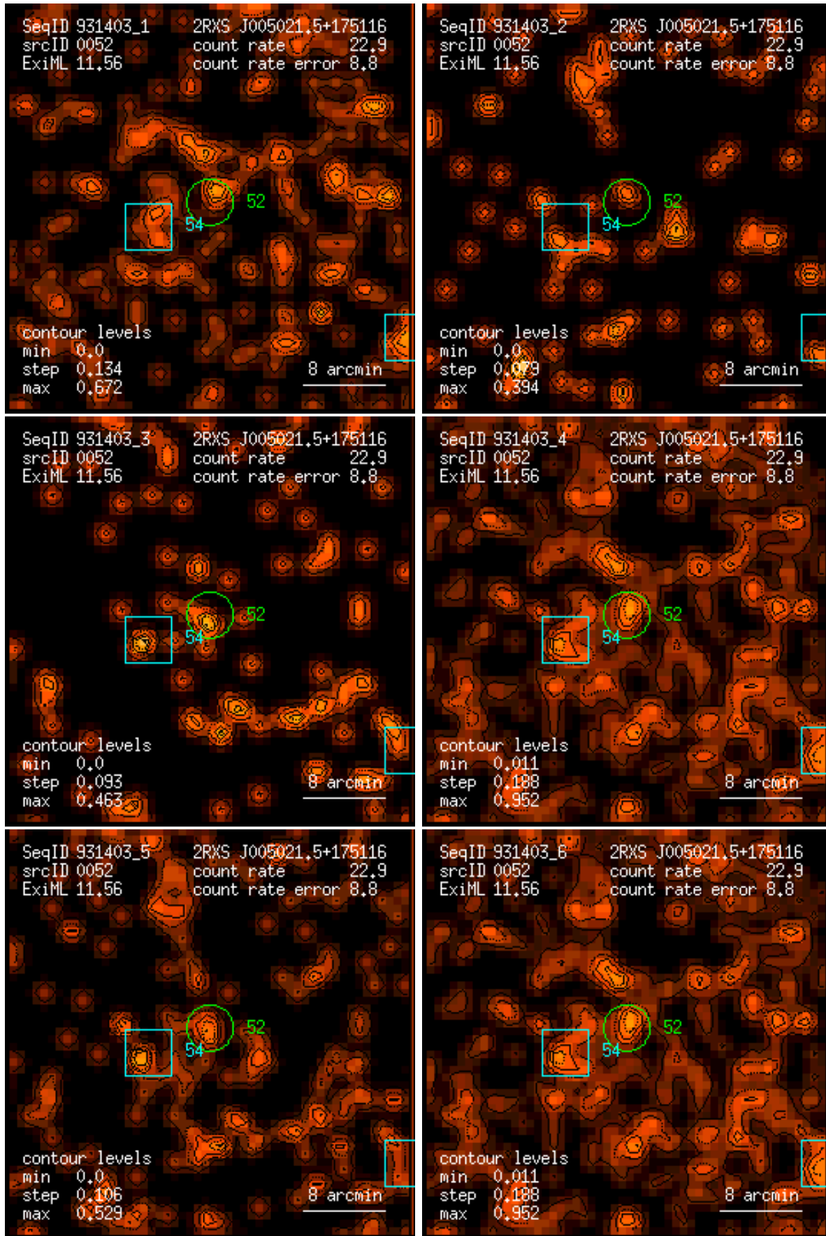
Figure 52: RASS 931403: detection 0052: band rate images, Gaussian filter: (1) PSPC channels 11 – 41, (2) 52 – 90, (3) 91 – 201, (4) 11 – 235, (5) 52 – 201, (6) 11 – 201. Broad band rates in counts/ks. Band rate contour levels in counts/ks/arcmin 2 .
