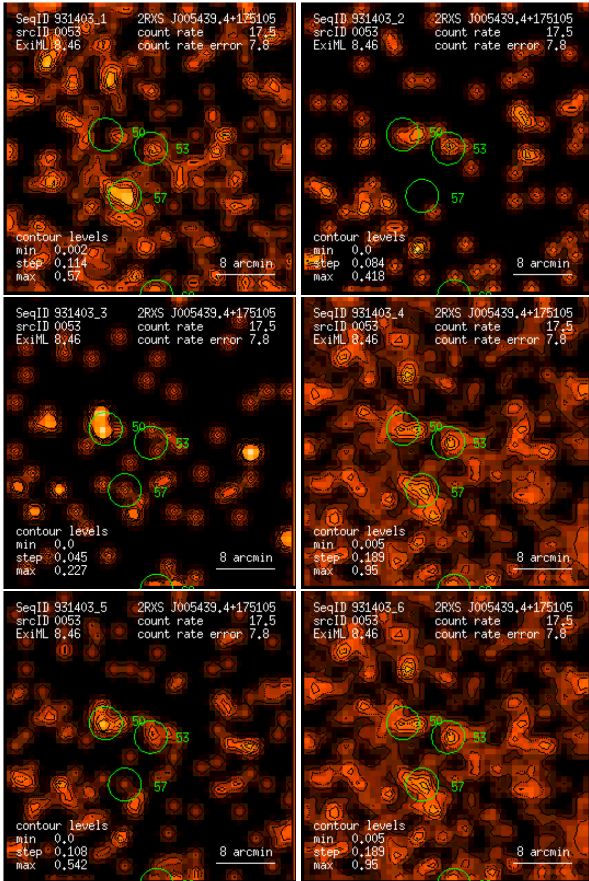
Figure 53: RASS 931403: detection 0053: band rate images, Gaussian filter: (1) PSPC channels 11 – 41, (2) 52 – 90, (3) 91 – 201, (4) 11 – 235, (5) 52 – 201, (6) 11 – 201. Broad band rates in counts/ks. Band rate contour levels in counts/ks/arcmin 2 .
