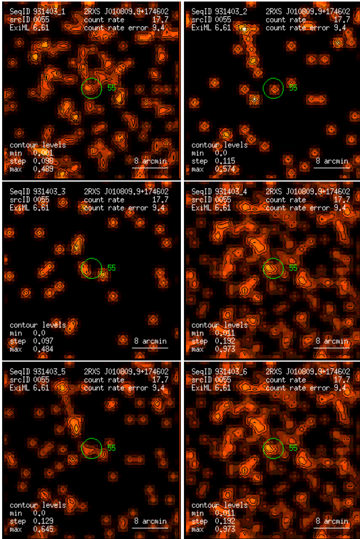
Figure 55: RASS 931403: detection 0055: band rate images, Gaussian filter: (1) PSPC channels 11 – 41, (2) 52 – 90, (3) 91 – 201, (4) 11 – 235, (5) 52 – 201, (6) 11 – 201. Broad band rates in counts/ks. Band rate contour levels in counts/ks/arcmin 2 .
