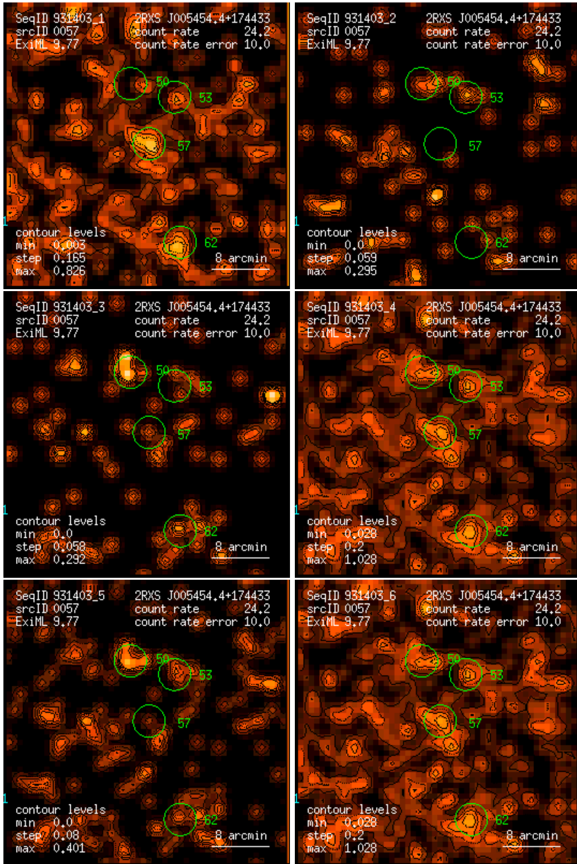
Figure 57: RASS 931403: detection 0057: band rate images, Gaussian filter: (1) PSPC channels 11 – 41, (2) 52 – 90, (3) 91 – 201, (4) 11 – 235, (5) 52 – 201, (6) 11 – 201. Broad band rates in counts/ks. Band rate contour levels in counts/ks/arcmin 2 .
