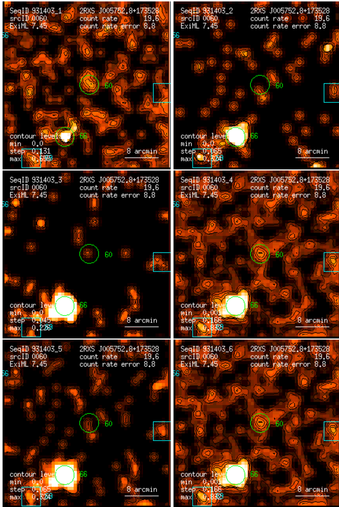
Figure 60: RASS 931403: detection 0060: band rate images, Gaussian filter: (1) PSPC channels 11 – 41, (2) 52 – 90, (3) 91 – 201, (4) 11 – 235, (5) 52 – 201, (6) 11 – 201. Broad band rates in counts/ks. Band rate contour levels in counts/ks/arcmin 2 .
