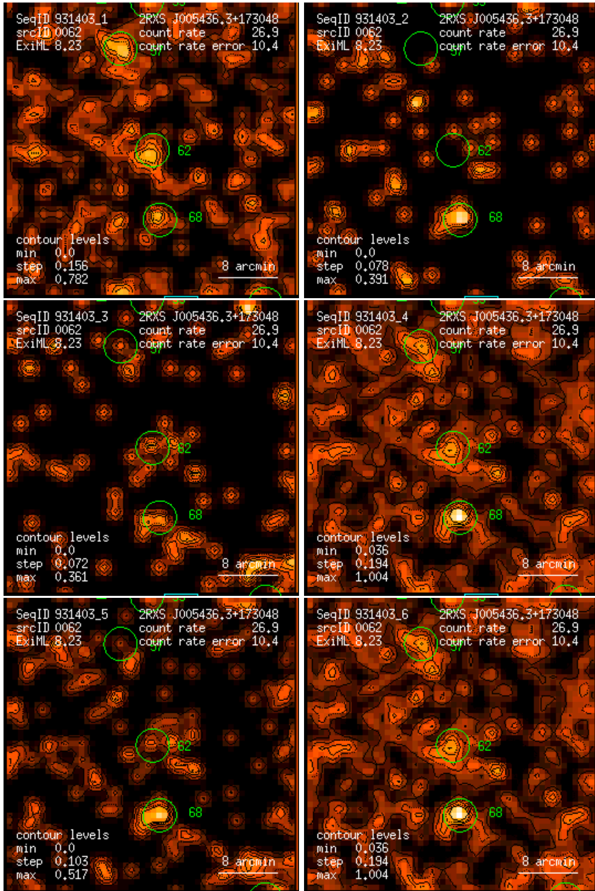
Figure 62: RASS 931403: detection 0062: band rate images, Gaussian filter: (1) PSPC channels 11 – 41, (2) 52 – 90, (3) 91 – 201, (4) 11 – 235, (5) 52 – 201, (6) 11 – 201. Broad band rates in counts/ks. Band rate contour levels in counts/ks/arcmin 2 .
