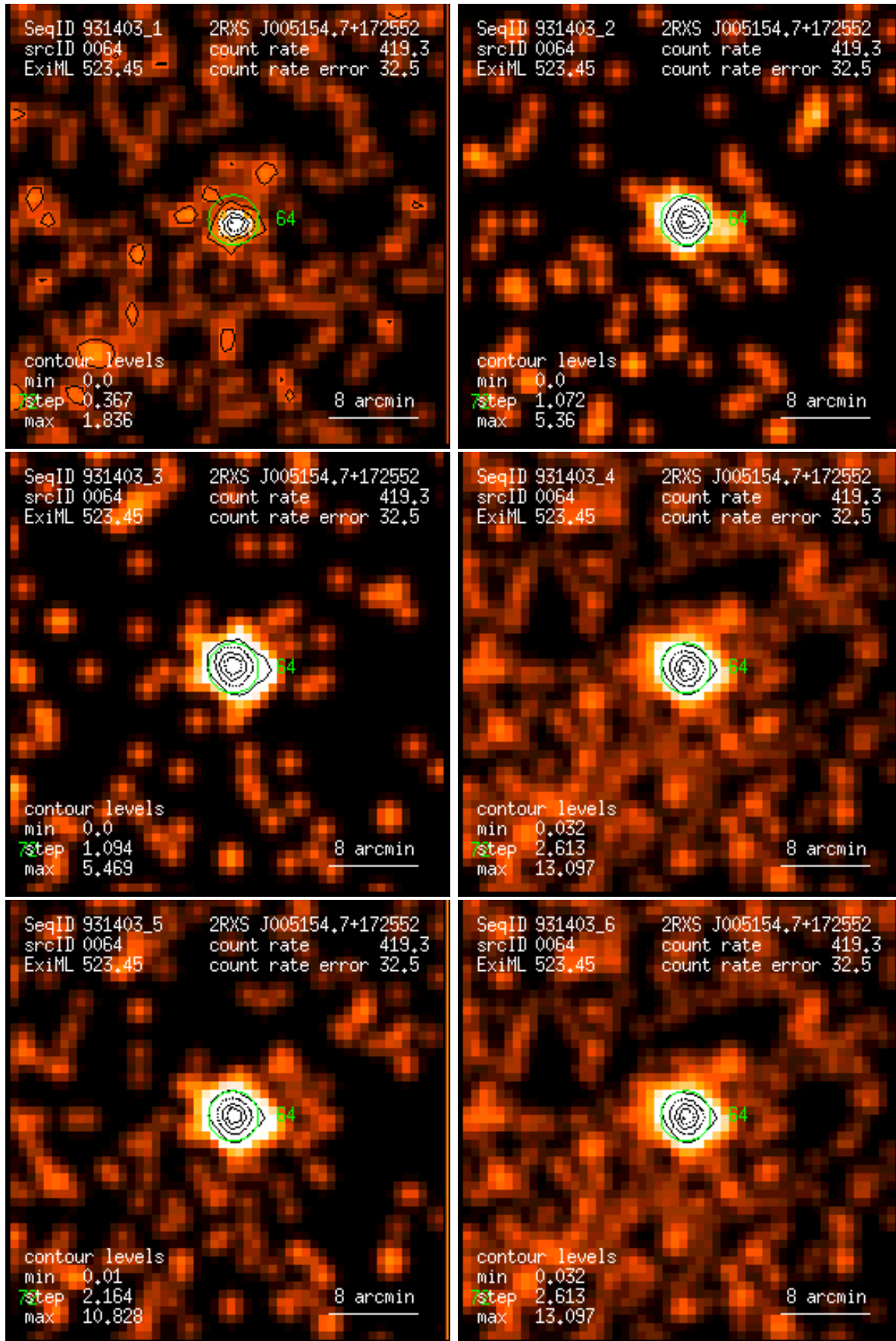
Figure 64: RASS 931403: detection 0064: band rate images, Gaussian filter: (1) PSPC channels 11 – 41, (2) 52 – 90, (3) 91 – 201, (4) 11 – 235, (5) 52 – 201, (6) 11 – 201. Broad band rates in counts/ks. Band rate contour levels in counts/ks/arcmin 2 .
