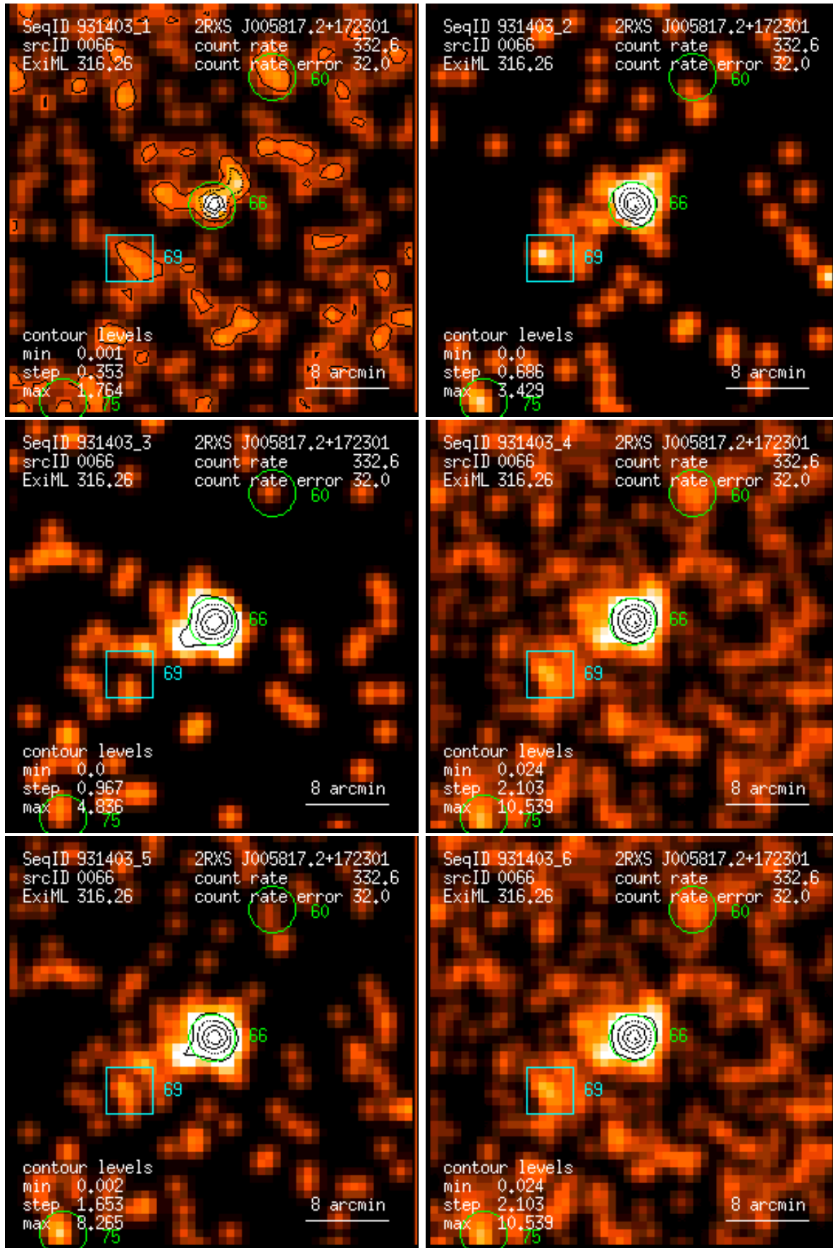
Figure 66: RASS 931403: detection 0066: band rate images, Gaussian filter: (1) PSPC channels 11 – 41, (2) 52 – 90, (3) 91 – 201, (4) 11 – 235, (5) 52 – 201, (6) 11 – 201. Broad band rates in counts/ks. Band rate contour levels in counts/ks/arcmin 2 .
