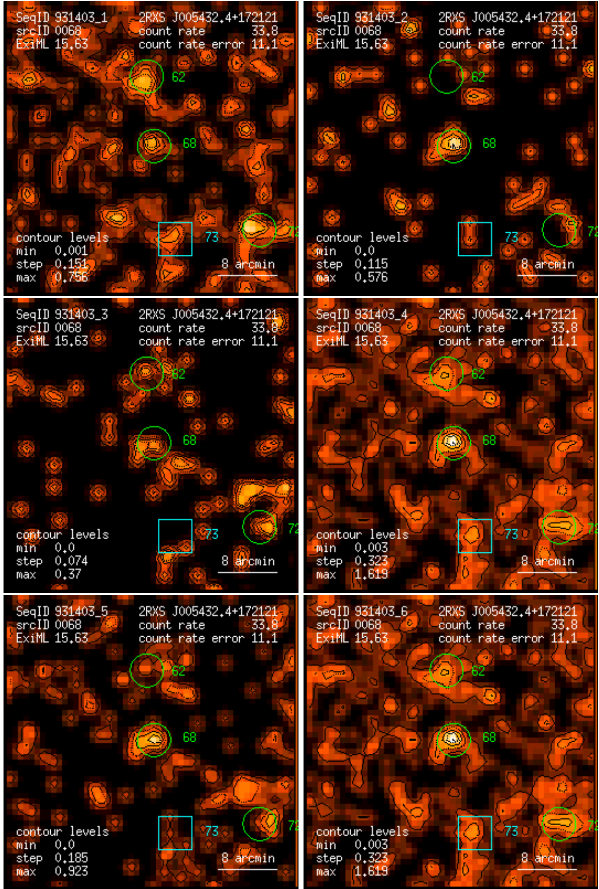
Figure 68: RASS 931403: detection 0068: band rate images, Gaussian filter: (1) PSPC channels 11 – 41, (2) 52 – 90, (3) 91 – 201, (4) 11 – 235, (5) 52 – 201, (6) 11 – 201. Broad band rates in counts/ks. Band rate contour levels in counts/ks/arcmin 2 .
