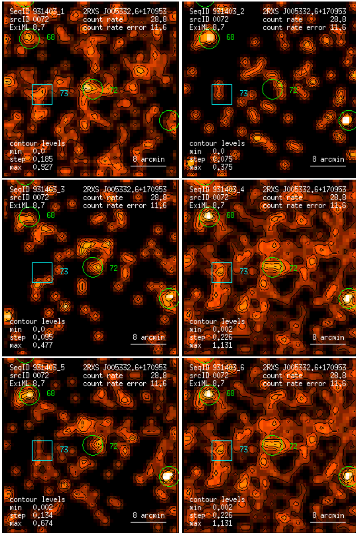
Figure 72: RASS 931403: detection 0072: band rate images, Gaussian filter: (1) PSPC channels 11 – 41, (2) 52 – 90, (3) 91 – 201, (4) 11 – 235, (5) 52 – 201, (6) 11 – 201. Broad band rates in counts/ks. Band rate contour levels in counts/ks/arcmin 2 .
