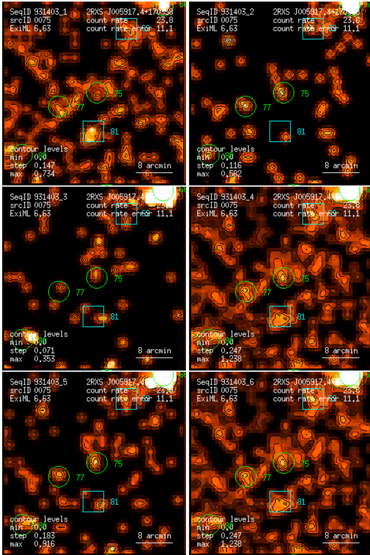
Figure 75: RASS 931403: detection 0075: band rate images, Gaussian filter: (1) PSPC channels 11 – 41, (2) 52 – 90, (3) 91 – 201, (4) 11 – 235, (5) 52 – 201, (6) 11 – 201. Broad band rates in counts/ks. Band rate contour levels in counts/ks/arcmin 2 .
