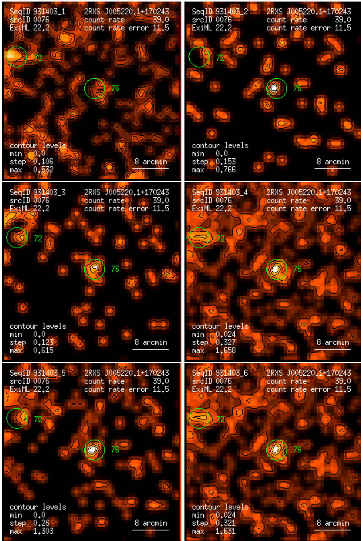
Figure 76: RASS 931403: detection 0076: band rate images, Gaussian filter: (1) PSPC channels 11 – 41, (2) 52 – 90, (3) 91 – 201, (4) 11 – 235, (5) 52 – 201, (6) 11 – 201. Broad band rates in counts/ks. Band rate contour levels in counts/ks/arcmin 2 .
