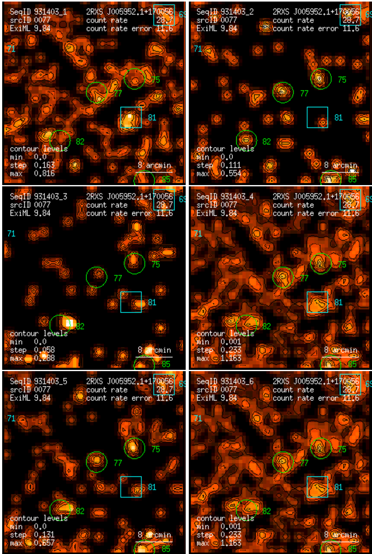
Figure 77: RASS 931403: detection 0077: band rate images, Gaussian filter: (1) PSPC channels 11 – 41, (2) 52 – 90, (3) 91 – 201, (4) 11 – 235, (5) 52 – 201, (6) 11 – 201. Broad band rates in counts/ks. Band rate contour levels in counts/ks/arcmin 2 .
