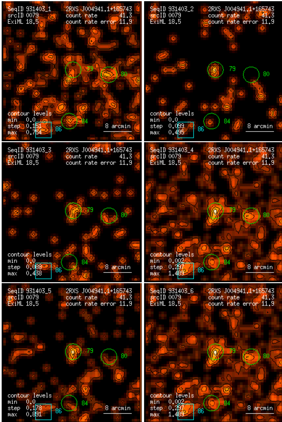
Figure 79: RASS 931403: detection 0079: band rate images, Gaussian filter: (1) PSPC channels 11 – 41, (2) 52 – 90, (3) 91 – 201, (4) 11 – 235, (5) 52 – 201, (6) 11 – 201. Broad band rates in counts/ks. Band rate contour levels in counts/ks/arcmin 2 .
