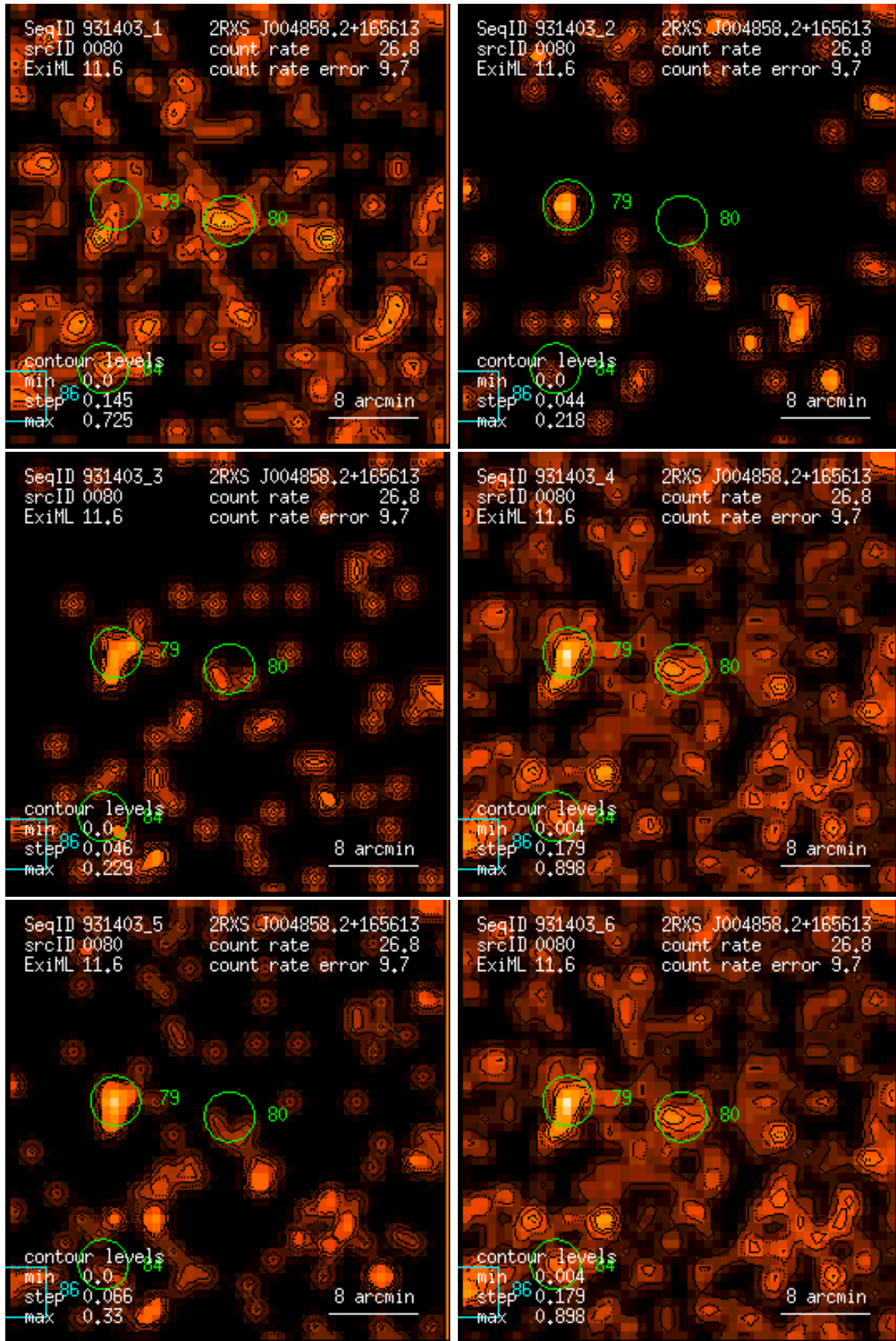
Figure 80: RASS 931403: detection 0080: band rate images, Gaussian filter: (1) PSPC channels 11 – 41, (2) 52 – 90, (3) 91 – 201, (4) 11 – 235, (5) 52 – 201, (6) 11 – 201. Broad band rates in counts/ks. Band rate contour levels in counts/ks/arcmin 2 .
