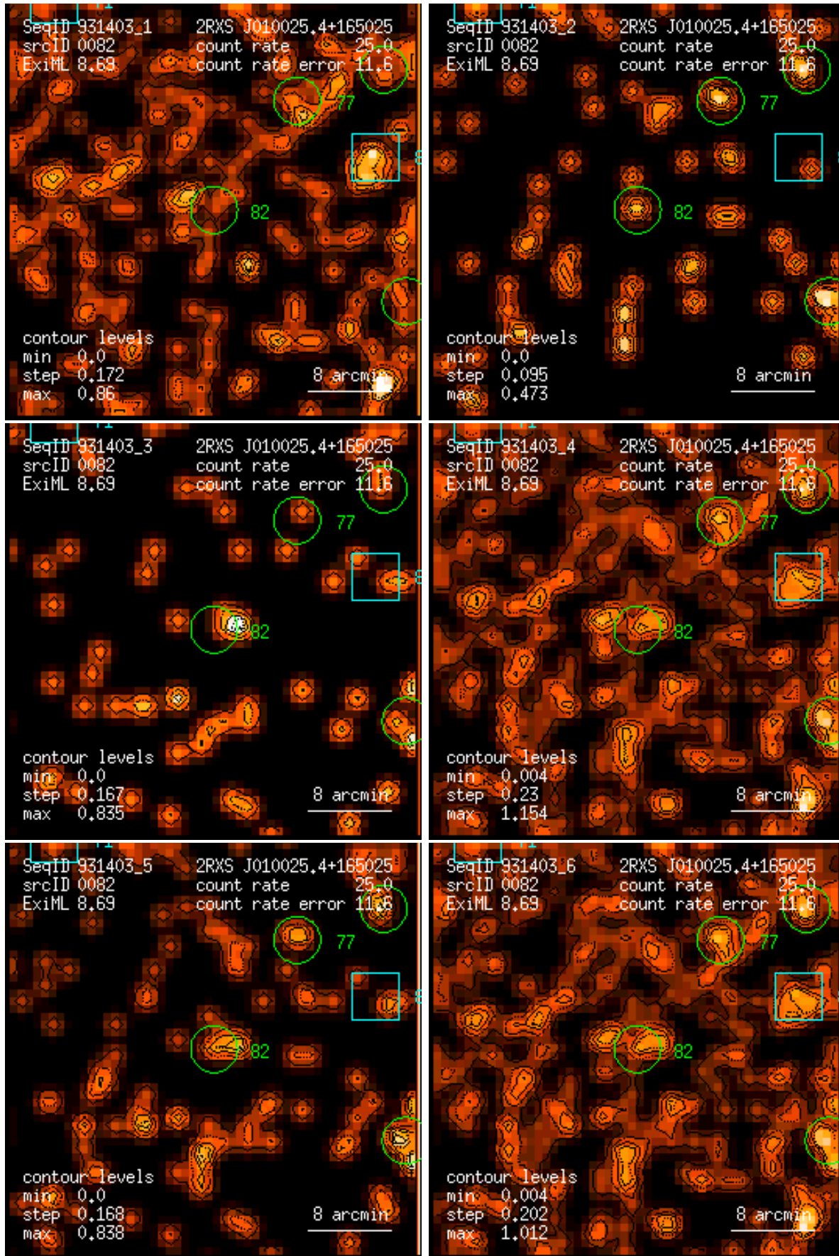
Figure 82: RASS 931403: detection 0082: band rate images, Gaussian filter: (1) PSPC channels 11 – 41, (2) 52 – 90, (3) 91 – 201, (4) 11 – 235, (5) 52 – 201, (6) 11 – 201. Broad band rates in counts/ks. Band rate contour levels in counts/ks/arcmin 2 .
