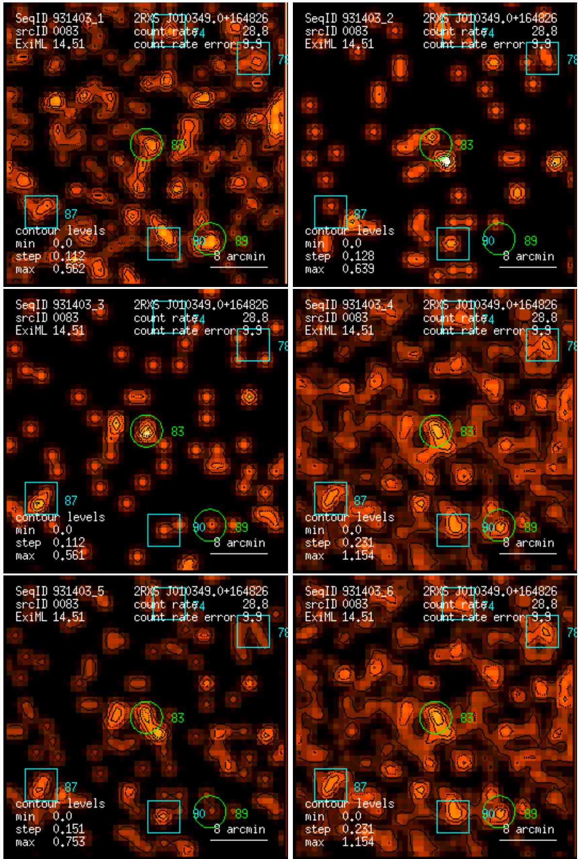
Figure 83: RASS 931403: detection 0083: band rate images, Gaussian filter: (1) PSPC channels 11 – 41, (2) 52 – 90, (3) 91 – 201, (4) 11 – 235, (5) 52 – 201, (6) 11 – 201. Broad band rates in counts/ks. Band rate contour levels in counts/ks/arcmin 2 .
