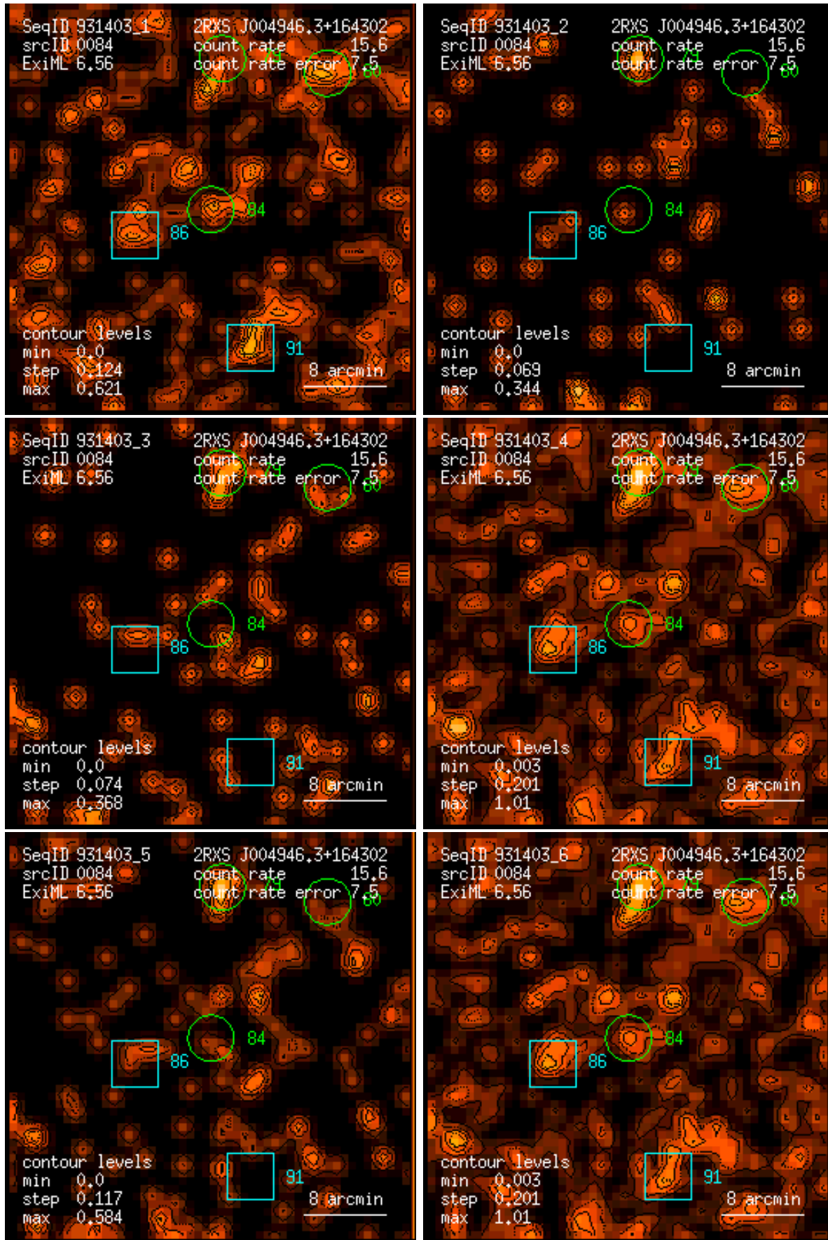
Figure 84: RASS 931403: detection 0084: band rate images, Gaussian filter: (1) PSPC channels 11 – 41, (2) 52 – 90, (3) 91 – 201, (4) 11 – 235, (5) 52 – 201, (6) 11 – 201. Broad band rates in counts/ks. Band rate contour levels in counts/ks/arcmin 2 .
