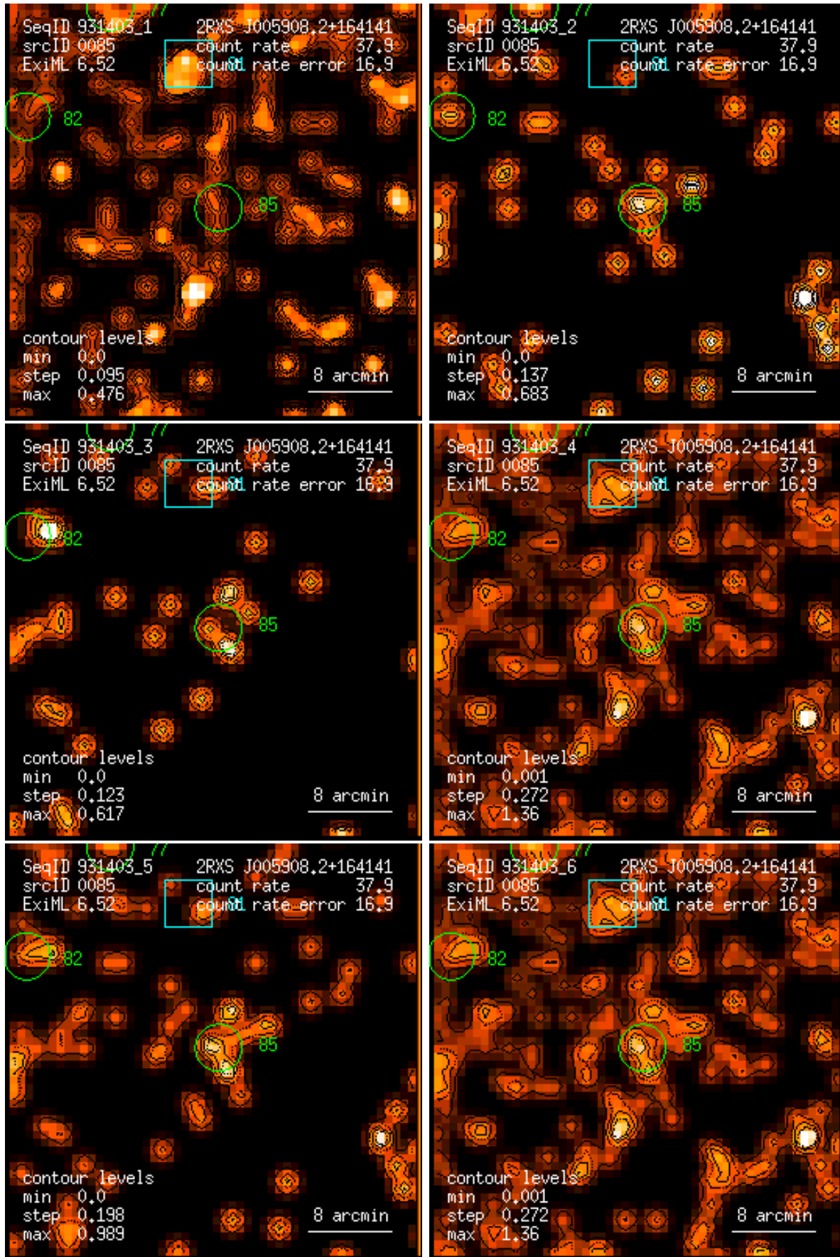
Figure 85: RASS 931403: detection 0085: band rate images, Gaussian filter: (1) PSPC channels 11 – 41, (2) 52 – 90, (3) 91 – 201, (4) 11 – 235, (5) 52 – 201, (6) 11 – 201. Broad band rates in counts/ks. Band rate contour levels in counts/ks/arcmin 2 .
