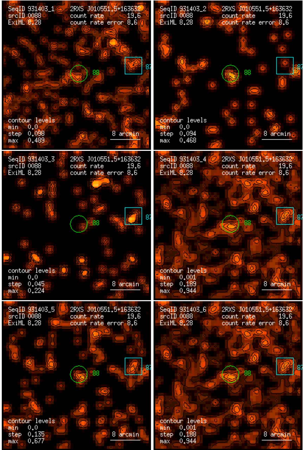
Figure 88: RASS 931403: detection 0088: band rate images, Gaussian filter: (1) PSPC channels 11 – 41, (2) 52 – 90, (3) 91 – 201, (4) 11 – 235, (5) 52 – 201, (6) 11 – 201. Broad band rates in counts/ks. Band rate contour levels in counts/ks/arcmin 2 .
