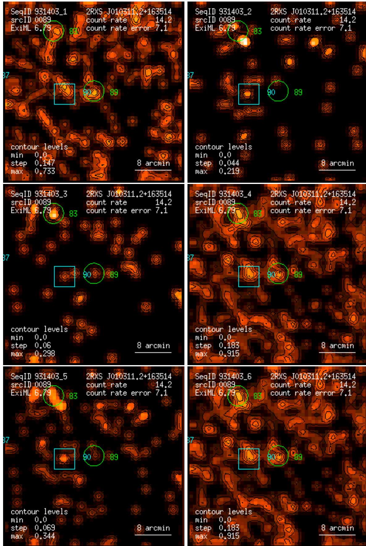
Figure 89: RASS 931403: detection 0089: band rate images, Gaussian filter: (1) PSPC channels 11 – 41, (2) 52 – 90, (3) 91 – 201, (4) 11 – 235, (5) 52 – 201, (6) 11 – 201. Broad band rates in counts/ks. Band rate contour levels in counts/ks/arcmin 2 .
