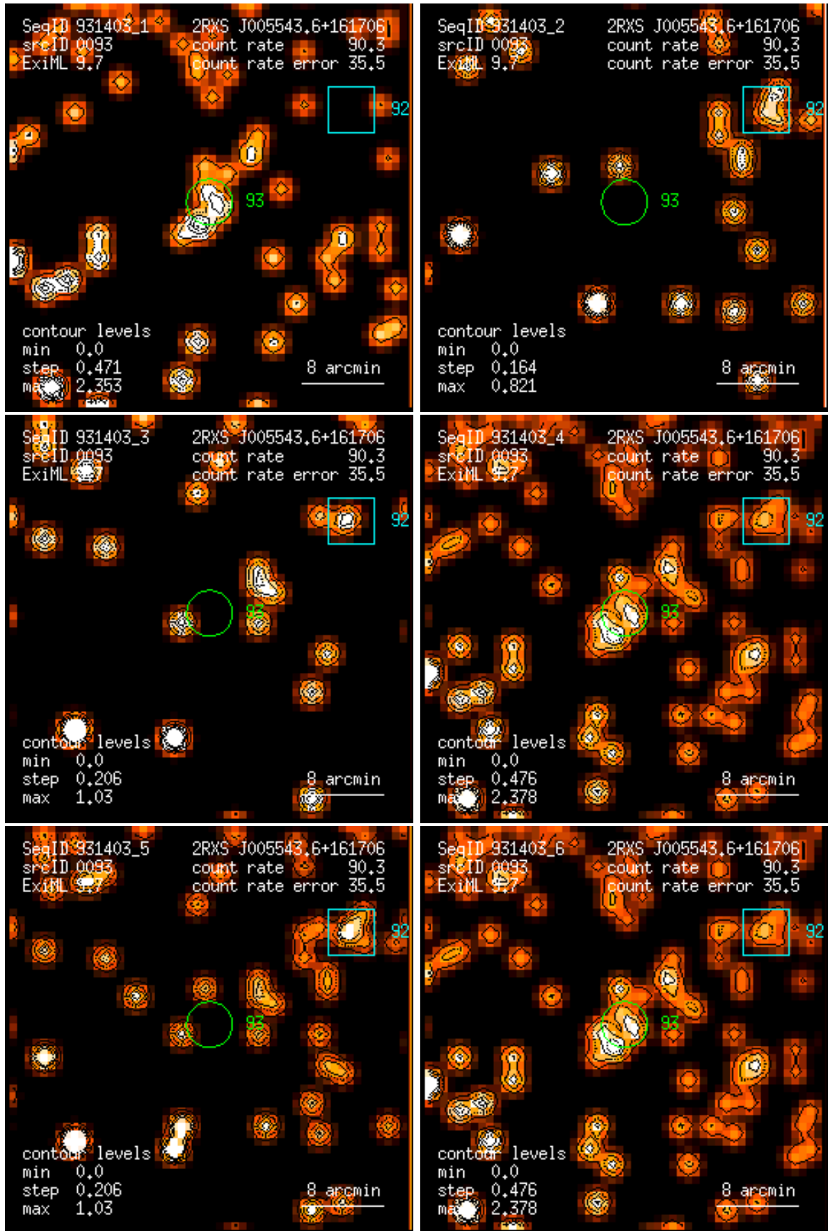
Figure 93: RASS 931403: detection 0093: band rate images, Gaussian filter: (1) PSPC channels 11 – 41, (2) 52 – 90, (3) 91 – 201, (4) 11 – 235, (5) 52 – 201, (6) 11 – 201. Broad band rates in counts/ks. Band rate contour levels in counts/ks/arcmin 2 .
