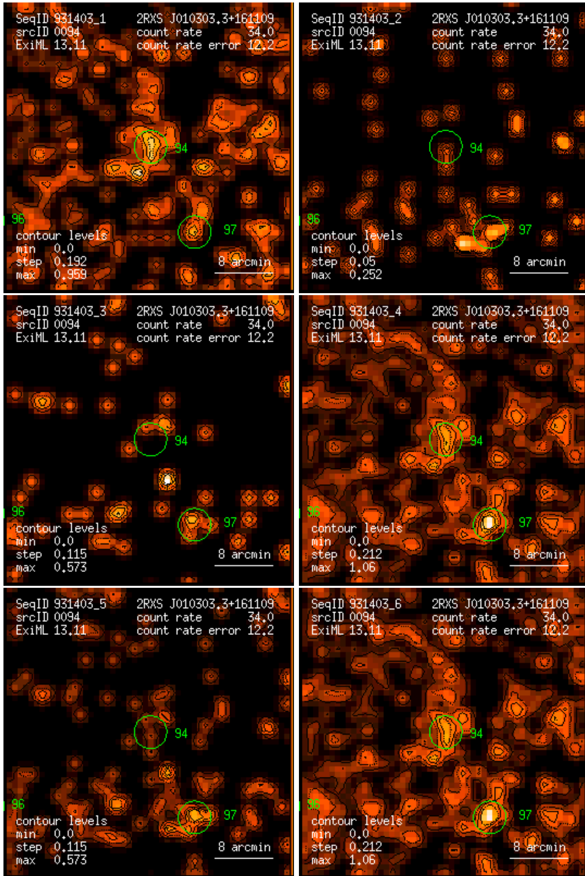
Figure 94: RASS 931403: detection 0094: band rate images, Gaussian filter: (1) PSPC channels 11 – 41, (2) 52 – 90, (3) 91 – 201, (4) 11 – 235, (5) 52 – 201, (6) 11 – 201. Broad band rates in counts/ks. Band rate contour levels in counts/ks/arcmin 2 .
