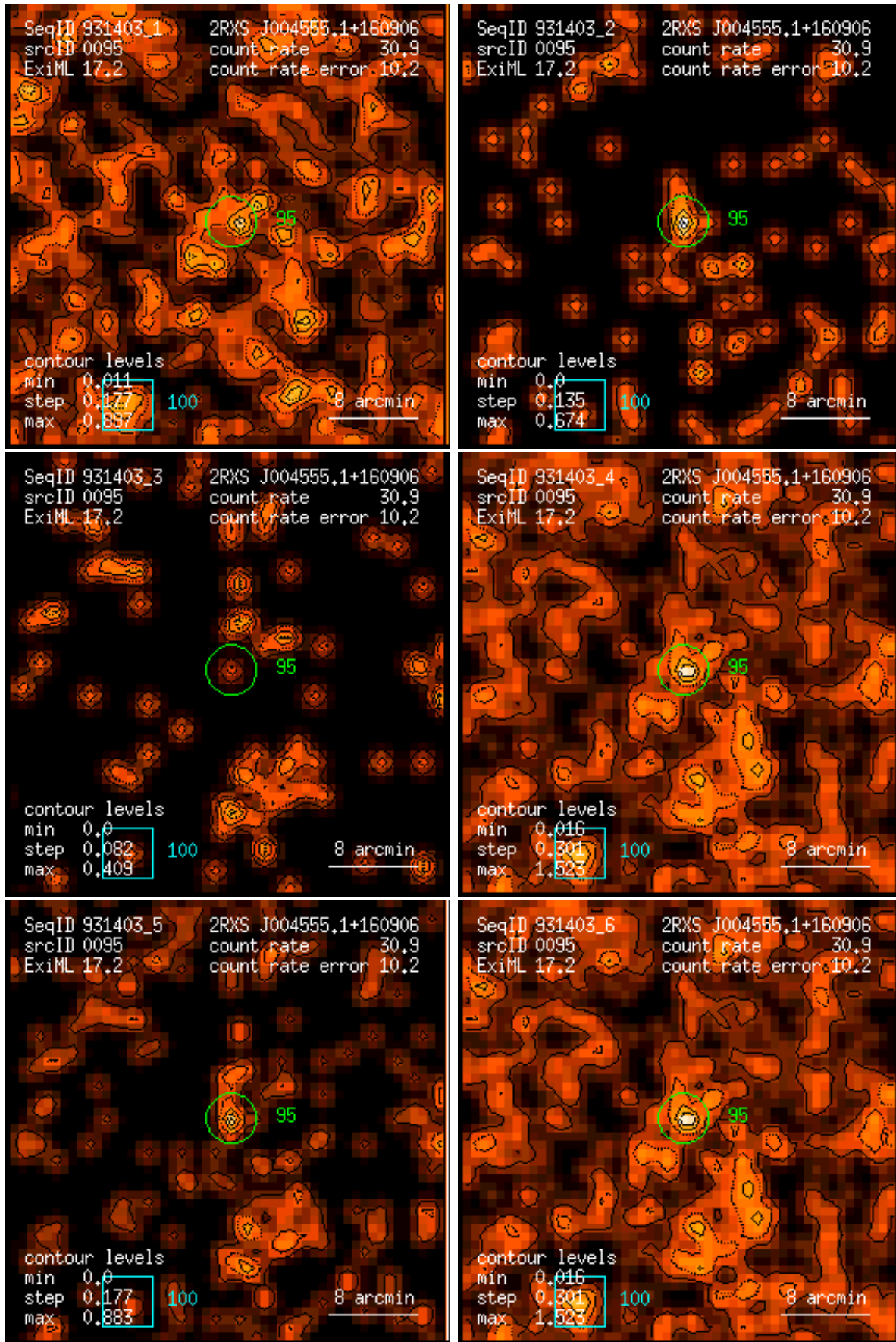
Figure 95: RASS 931403: detection 0095: band rate images, Gaussian filter: (1) PSPC channels 11 – 41, (2) 52 – 90, (3) 91 – 201, (4) 11 – 235, (5) 52 – 201, (6) 11 – 201. Broad band rates in counts/ks. Band rate contour levels in counts/ks/arcmin 2 .
