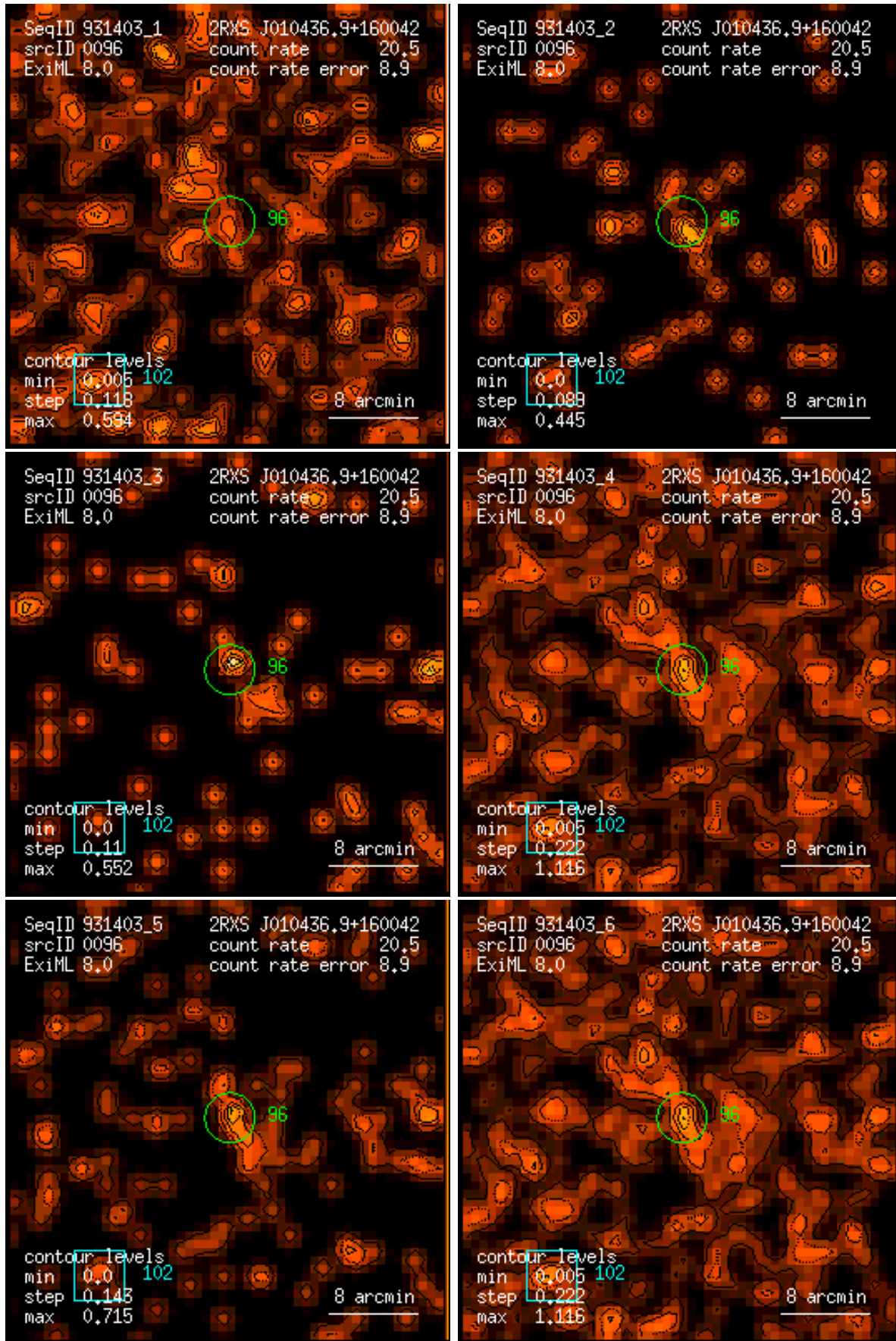
Figure 96: RASS 931403: detection 0096: band rate images, Gaussian filter: (1) PSPC channels 11 – 41, (2) 52 – 90, (3) 91 – 201, (4) 11 – 235, (5) 52 – 201, (6) 11 – 201. Broad band rates in counts/ks. Band rate contour levels in counts/ks/arcmin 2 .
