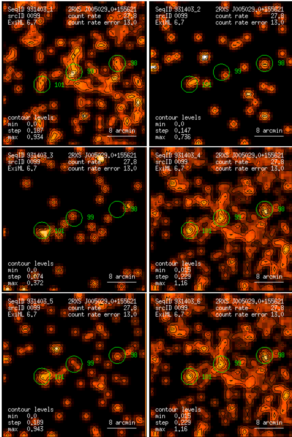
Figure 99: RASS 931403: detection 0099: band rate images, Gaussian filter: (1) PSPC channels 11 – 41, (2) 52 – 90, (3) 91 – 201, (4) 11 – 235, (5) 52 – 201, (6) 11 – 201. Broad band rates in counts/ks. Band rate contour levels in counts/ks/arcmin 2 .
