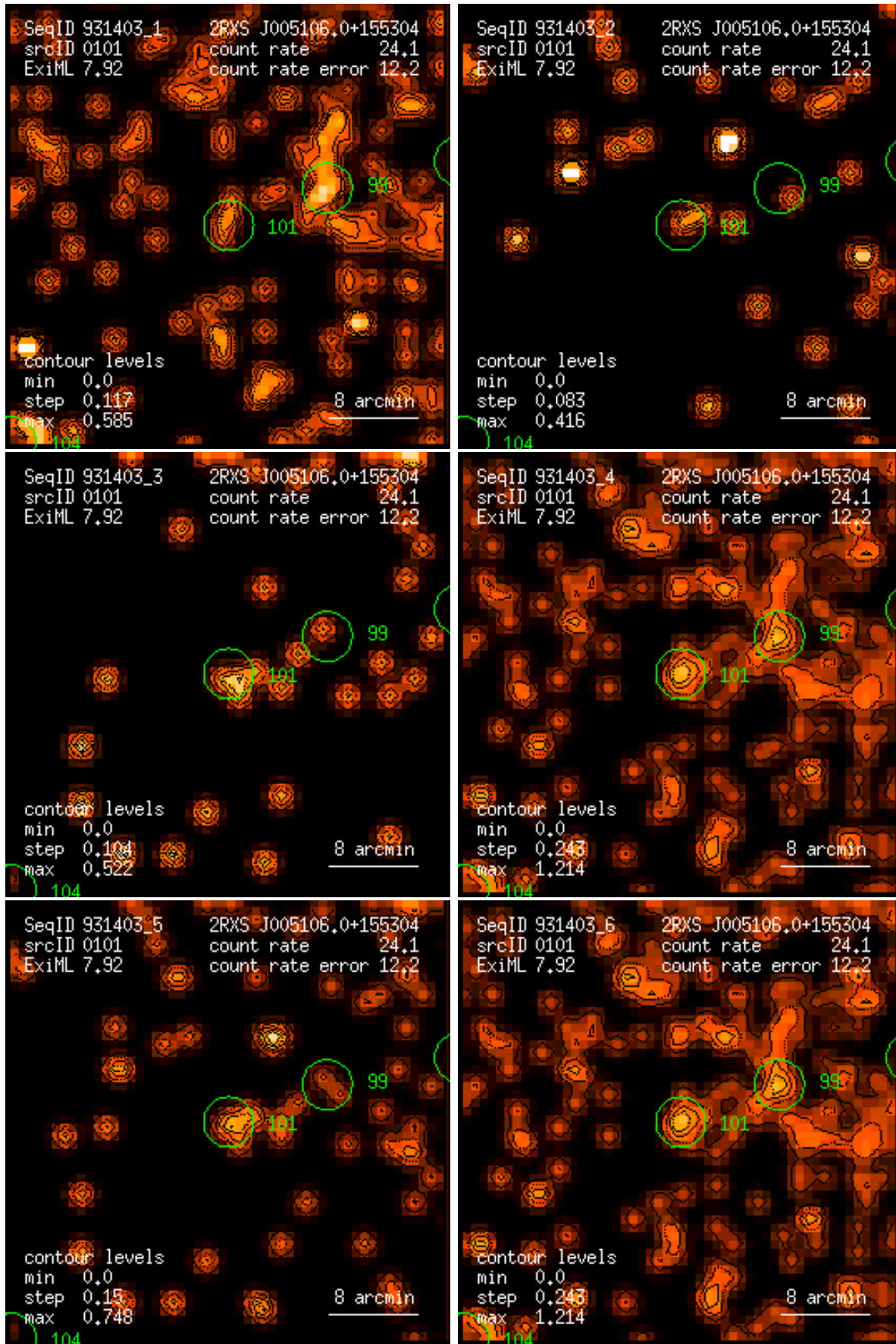
Figure 101: RASS 931403: detection 0101: band rate images, Gaussian filter: (1) PSPC channels 11 – 41, (2) 52 – 90, (3) 91 – 201, (4) 11 – 235, (5) 52 – 201, (6) 11 – 201. Broad band rates in counts/ks. Band rate contour levels in counts/ks/arcmin 2 .
