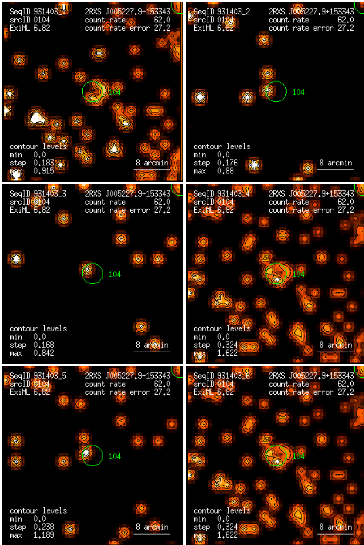
Figure 104: RASS 931403: detection 0104: band rate images, Gaussian filter: (1) PSPC channels 11 – 41, (2) 52 – 90, (3) 91 – 201, (4) 11 – 235, (5) 52 – 201, (6) 11 – 201. Broad band rates in counts/ks. Band rate contour levels in counts/ks/arcmin 2 .
