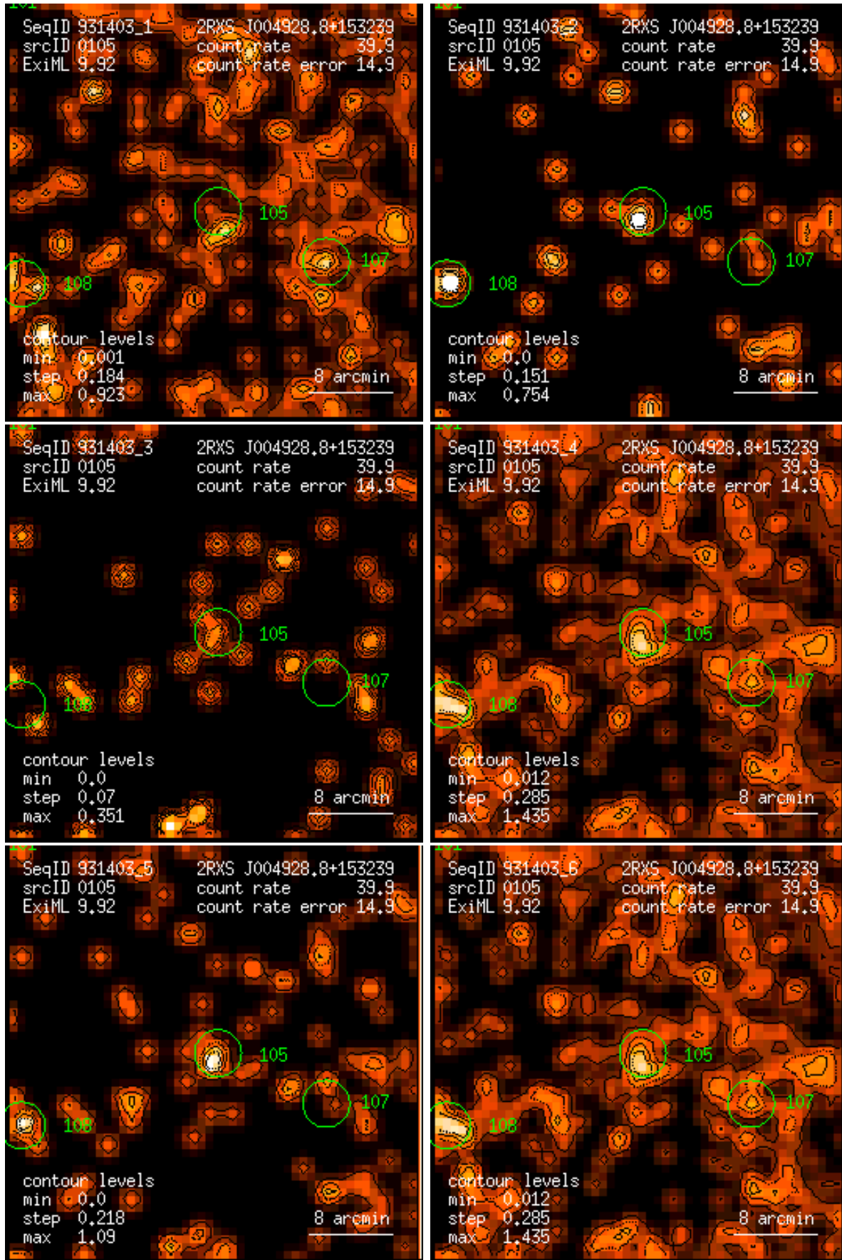
Figure 105: RASS 931403: detection 0105: band rate images, Gaussian filter: (1) PSPC channels 11 – 41, (2) 52 – 90, (3) 91 – 201, (4) 11 – 235, (5) 52 – 201, (6) 11 – 201. Broad band rates in counts/ks. Band rate contour levels in counts/ks/arcmin 2 .
