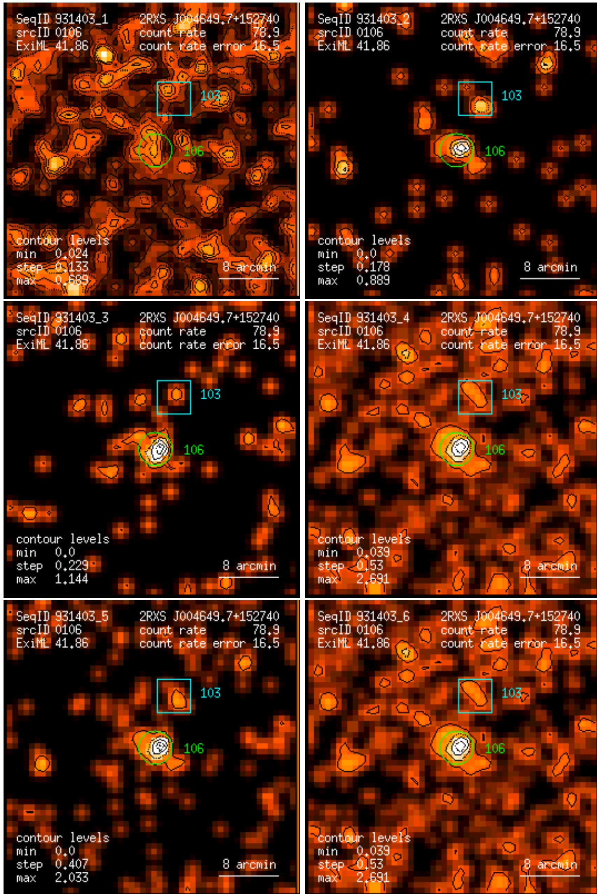
Figure 106: RASS 931403: detection 0106: band rate images, Gaussian filter: (1) PSPC channels 11 – 41, (2) 52 – 90, (3) 91 – 201, (4) 11 – 235, (5) 52 – 201, (6) 11 – 201. Broad band rates in counts/ks. Band rate contour levels in counts/ks/arcmin 2 .
