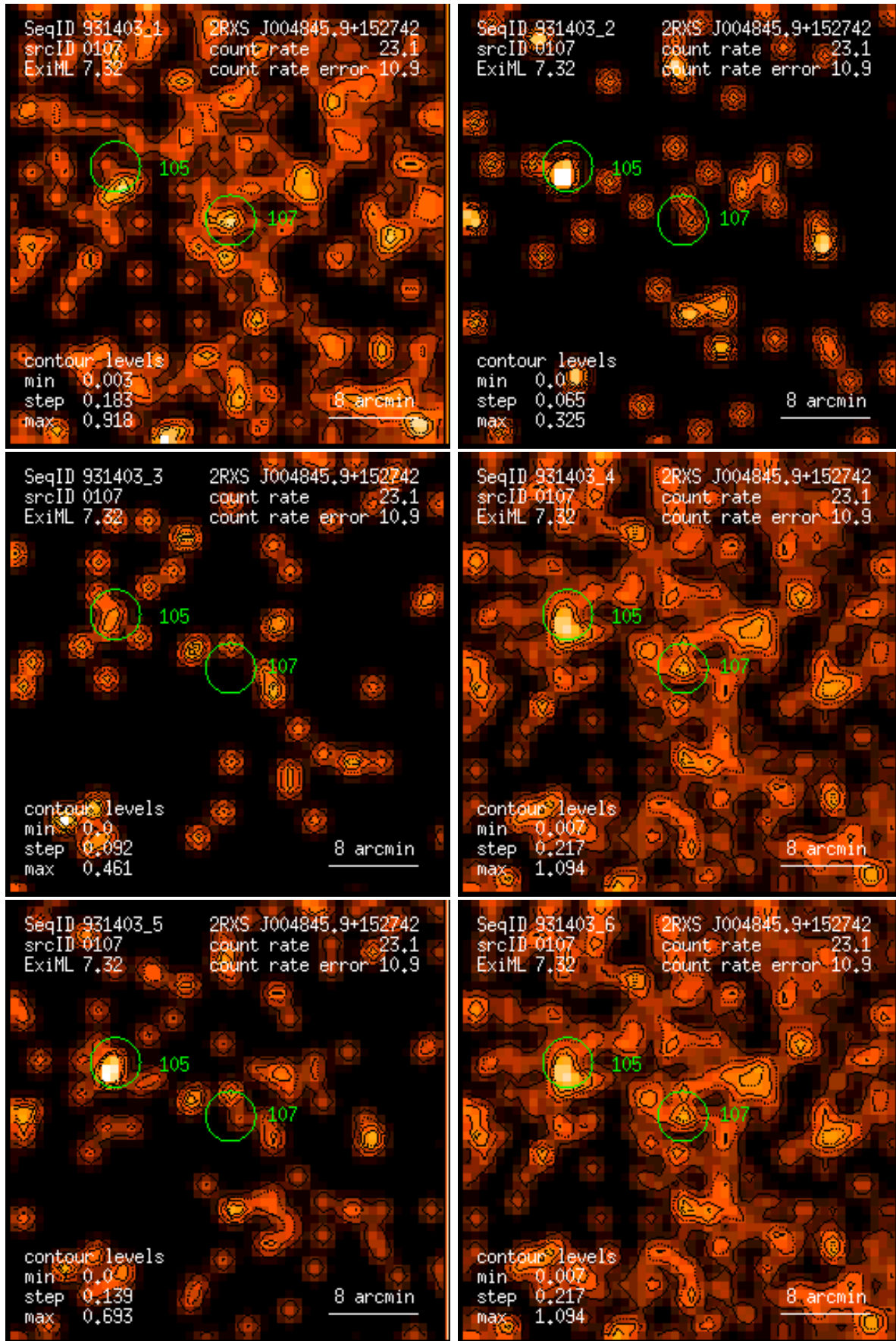
Figure 107: RASS 931403: detection 0107: band rate images, Gaussian filter: (1) PSPC channels 11 – 41, (2) 52 – 90, (3) 91 – 201, (4) 11 – 235, (5) 52 – 201, (6) 11 – 201. Broad band rates in counts/ks. Band rate contour levels in counts/ks/arcmin 2 .
