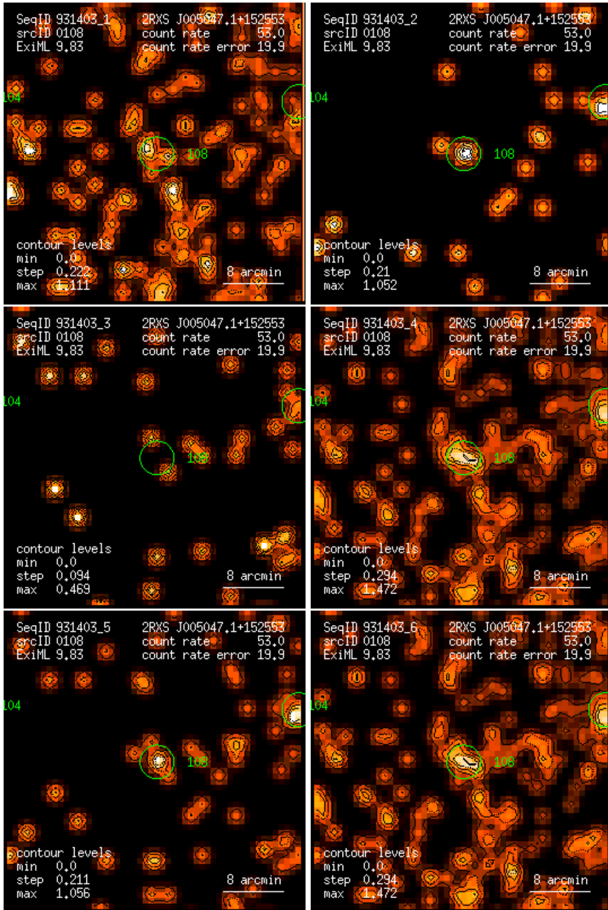
Figure 108: RASS 931403: detection 0108: band rate images, Gaussian filter: (1) PSPC channels 11 – 41, (2) 52 – 90, (3) 91 – 201, (4) 11 – 235, (5) 52 – 201, (6) 11 – 201. Broad band rates in counts/ks. Band rate contour levels in counts/ks/arcmin 2 .
