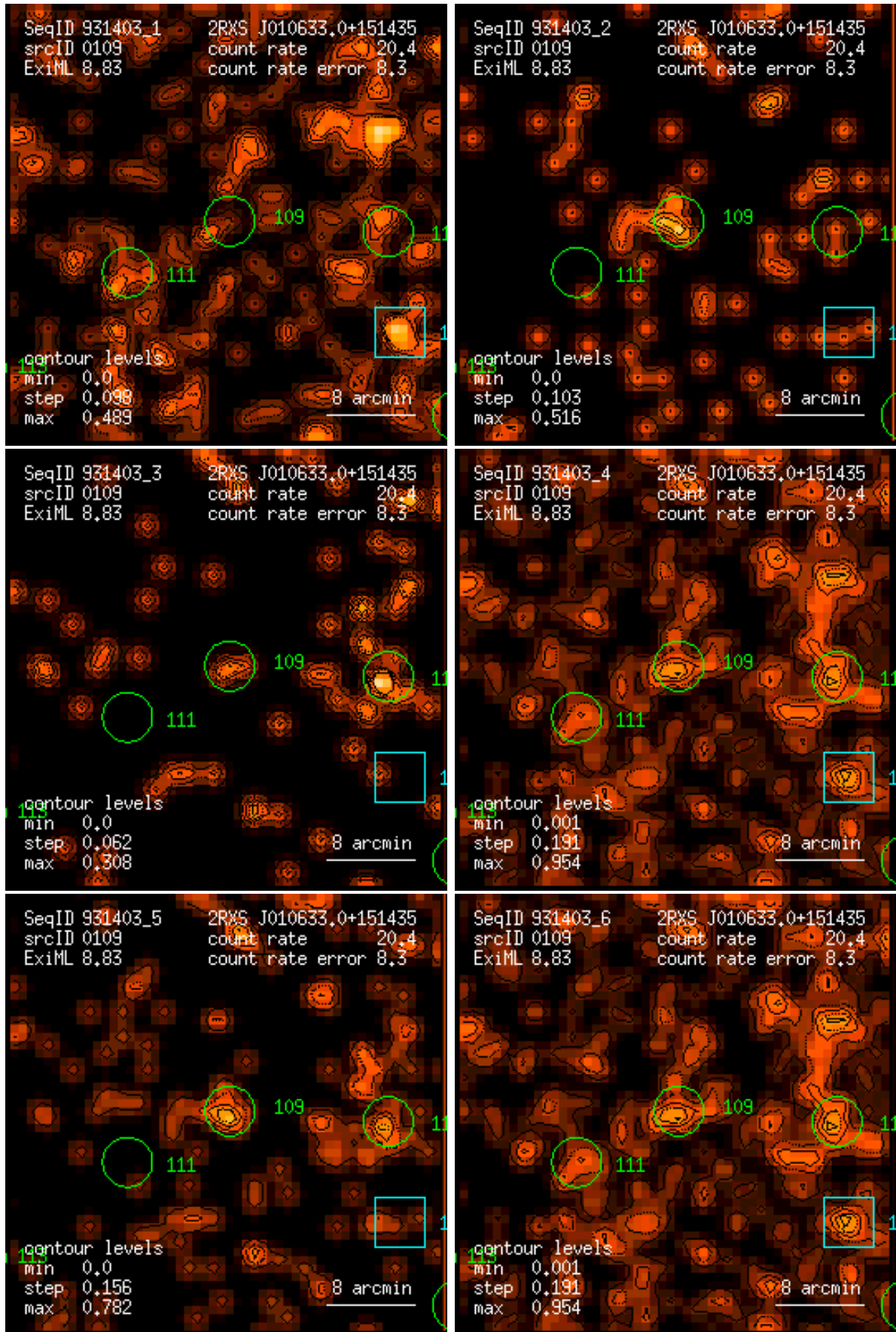
Figure 109: RASS 931403: detection 0109: band rate images, Gaussian filter: (1) PSPC channels 11 – 41, (2) 52 – 90, (3) 91 – 201, (4) 11 – 235, (5) 52 – 201, (6) 11 – 201. Broad band rates in counts/ks. Band rate contour levels in counts/ks/arcmin 2 .
