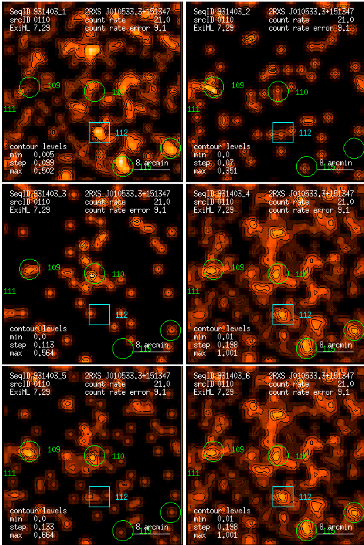
Figure 110: RASS 931403: detection 0110: band rate images, Gaussian filter: (1) PSPC channels 11 – 41, (2) 52 – 90, (3) 91 – 201, (4) 11 – 235, (5) 52 – 201, (6) 11 – 201. Broad band rates in counts/ks. Band rate contour levels in counts/ks/arcmin 2 .
