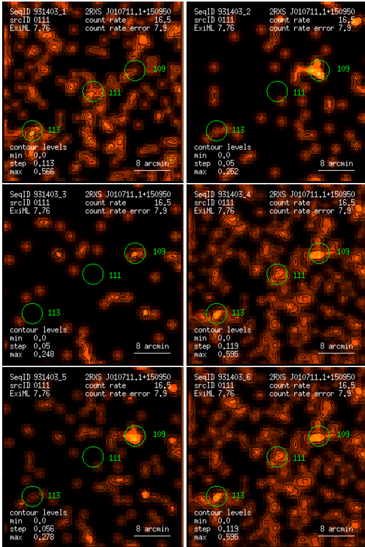
Figure 111: RASS 931403: detection 0111: band rate images, Gaussian filter: (1) PSPC channels 11 – 41, (2) 52 – 90, (3) 91 – 201, (4) 11 – 235, (5) 52 – 201, (6) 11 – 201. Broad band rates in counts/ks. Band rate contour levels in counts/ks/arcmin 2 .
