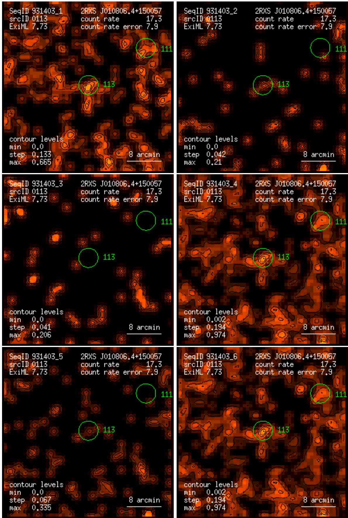
Figure 113: RASS 931403: detection 0113: band rate images, Gaussian filter: (1) PSPC channels 11 – 41, (2) 52 – 90, (3) 91 – 201, (4) 11 – 235, (5) 52 – 201, (6) 11 – 201. Broad band rates in counts/ks. Band rate contour levels in counts/ks/arcmin 2 .
