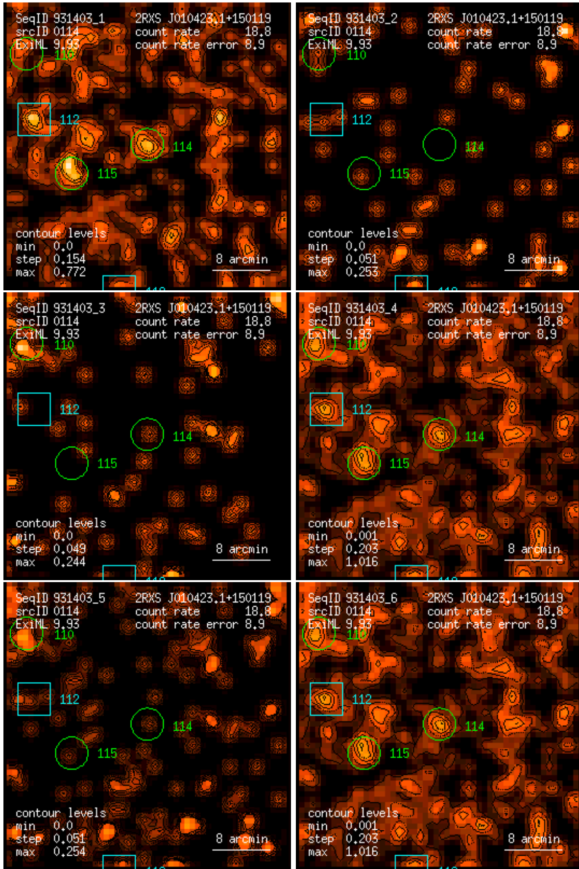
Figure 114: RASS 931403: detection 0114: band rate images, Gaussian filter: (1) PSPC channels 11 – 41, (2) 52 – 90, (3) 91 – 201, (4) 11 – 235, (5) 52 – 201, (6) 11 – 201. Broad band rates in counts/ks. Band rate contour levels in counts/ks/arcmin 2 .
