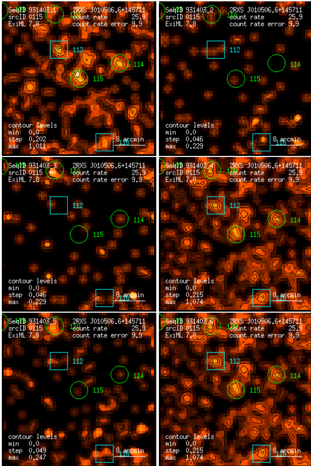
Figure 115: RASS 931403: detection 0115: band rate images, Gaussian filter: (1) PSPC channels 11 – 41, (2) 52 – 90, (3) 91 – 201, (4) 11 – 235, (5) 52 – 201, (6) 11 – 201. Broad band rates in counts/ks. Band rate contour levels in counts/ks/arcmin 2 .
