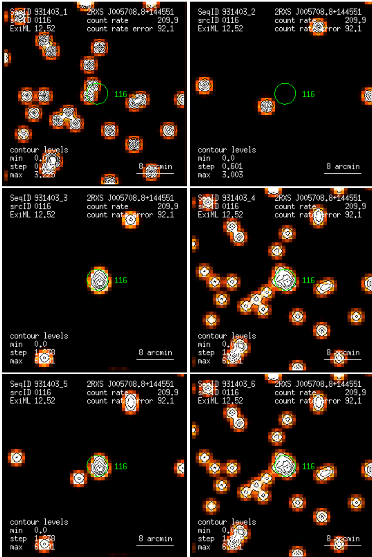
Figure 116: RASS 931403: detection 0116: band rate images, Gaussian filter: (1) PSPC channels 11 – 41, (2) 52 – 90, (3) 91 – 201, (4) 11 – 235, (5) 52 – 201, (6) 11 – 201. Broad band rates in counts/ks. Band rate contour levels in counts/ks/arcmin 2 .
