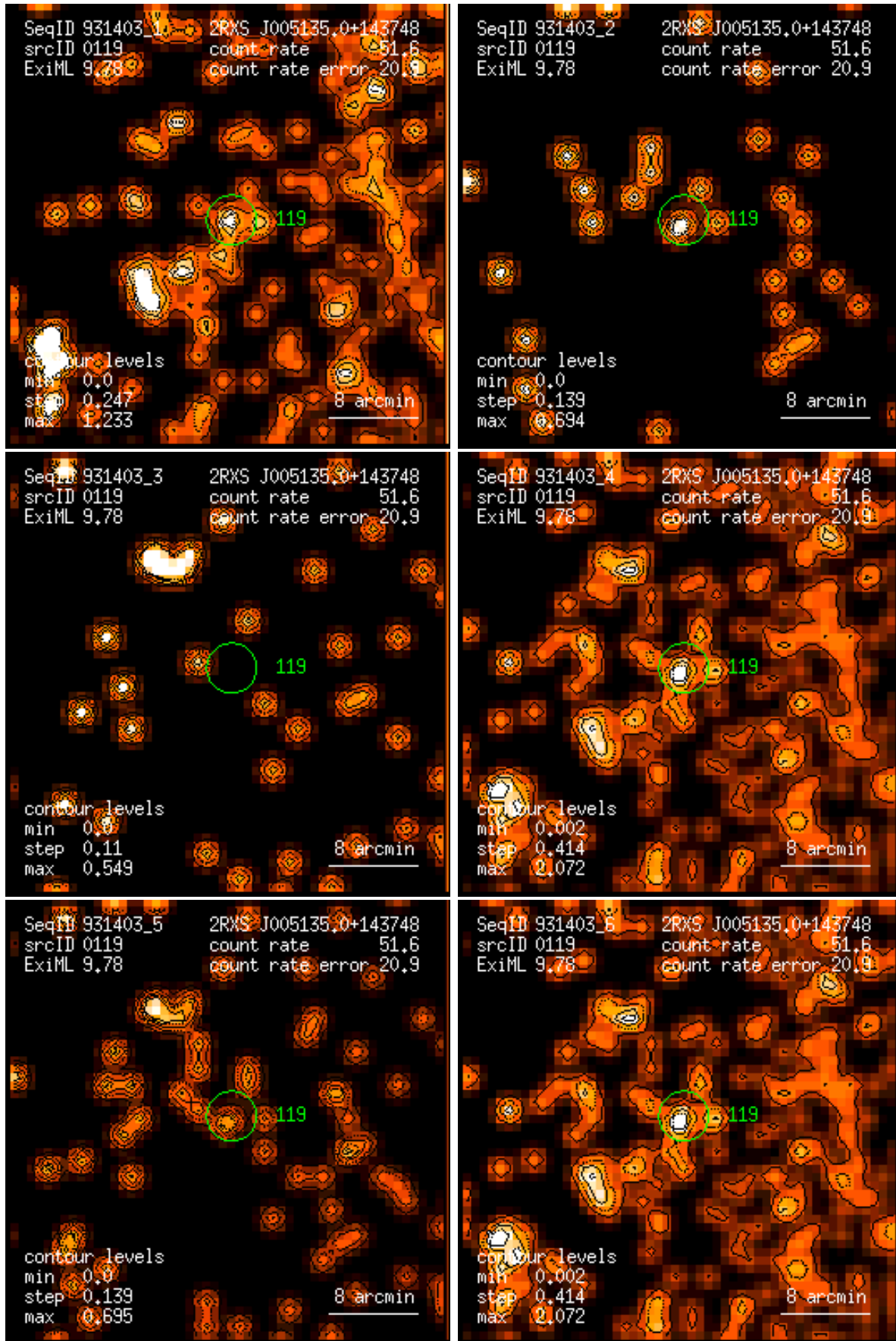
Figure 119: RASS 931403: detection 0119: band rate images, Gaussian filter: (1) PSPC channels 11 – 41, (2) 52 – 90, (3) 91 – 201, (4) 11 – 235, (5) 52 – 201, (6) 11 – 201. Broad band rates in counts/ks. Band rate contour levels in counts/ks/arcmin 2 .
