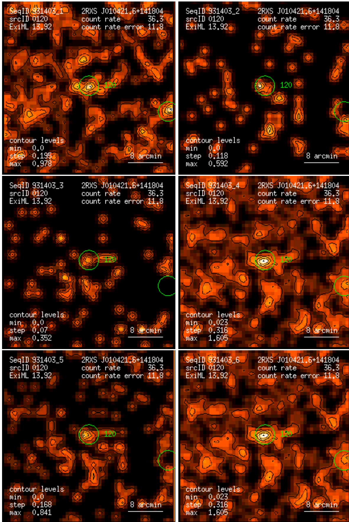
Figure 120: RASS 931403: detection 0120: band rate images, Gaussian filter: (1) PSPC channels 11 – 41, (2) 52 – 90, (3) 91 – 201, (4) 11 – 235, (5) 52 – 201, (6) 11 – 201. Broad band rates in counts/ks. Band rate contour levels in counts/ks/arcmin 2 .
