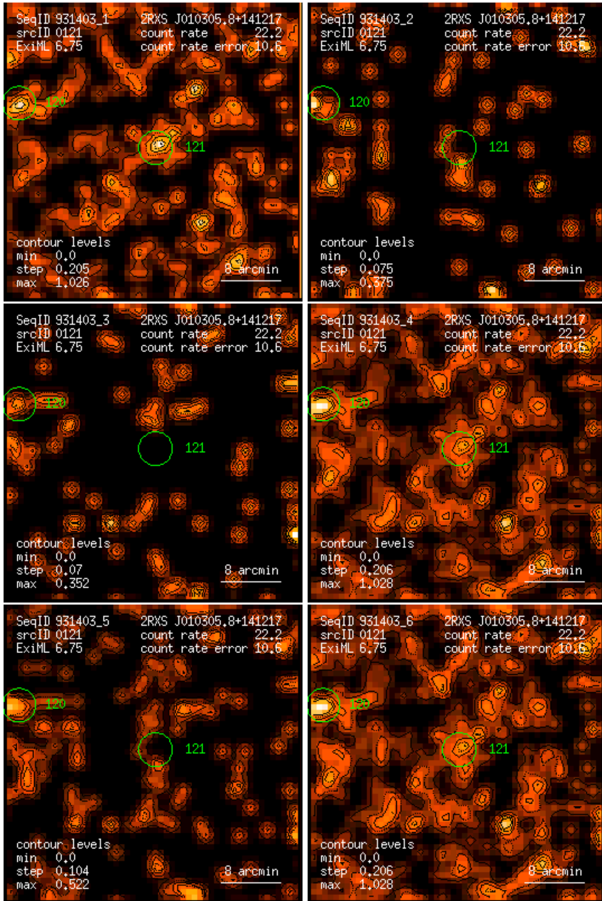
Figure 121: RASS 931403: detection 0121: band rate images, Gaussian filter: (1) PSPC channels 11 – 41, (2) 52 – 90, (3) 91 – 201, (4) 11 – 235, (5) 52 – 201, (6) 11 – 201. Broad band rates in counts/ks. Band rate contour levels in counts/ks/arcmin 2 .
