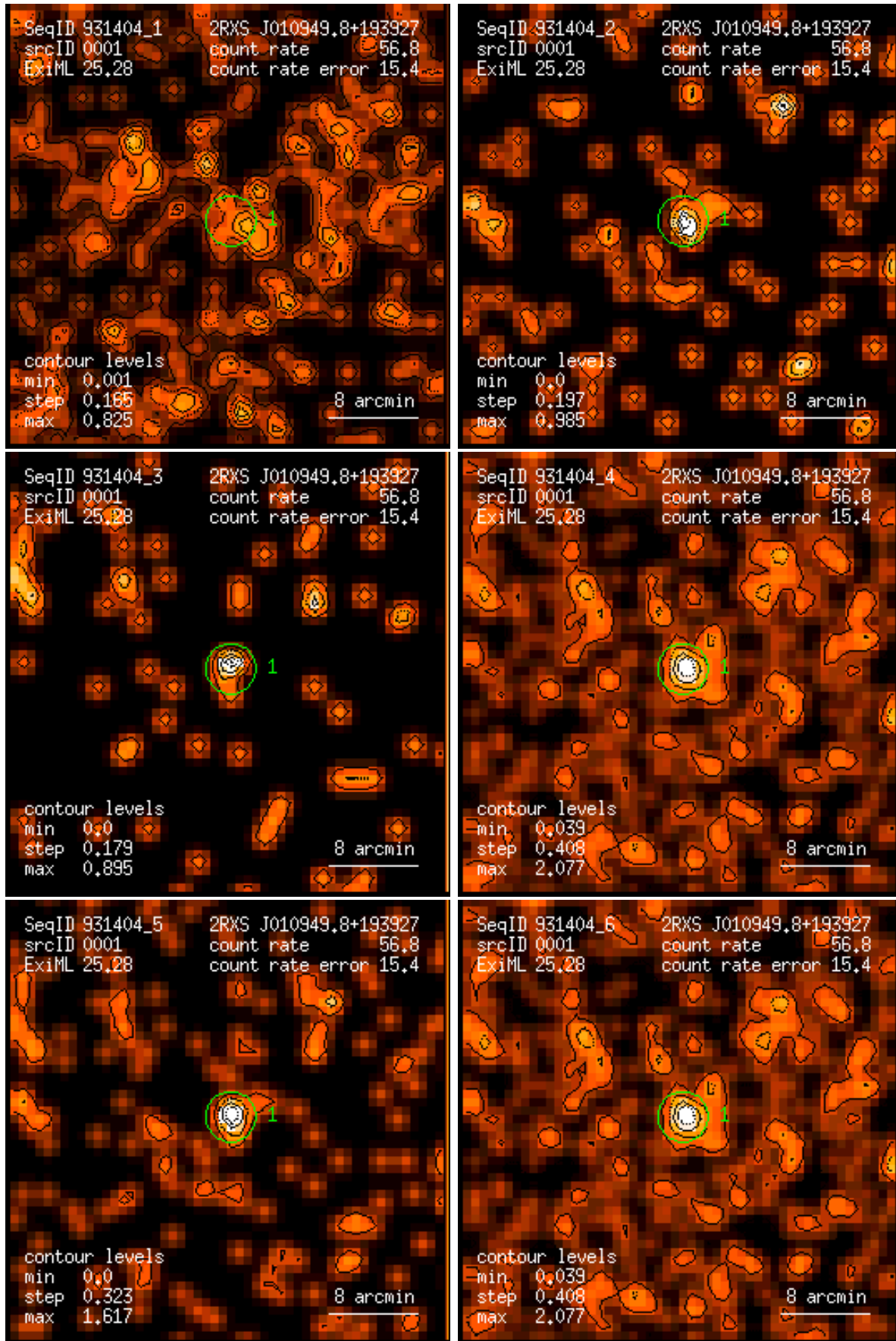
Figure 1: RASS 931404: detection 0001: band rate images, Gaussian filter: (1) PSPC channels 11 – 41, (2) 52 – 90, (3) 91 – 201, (4) 11 – 235, (5) 52 – 201, (6) 11 – 201. Broad band rates in counts/ks. Band rate contour levels in counts/ks/arcmin 2 .
