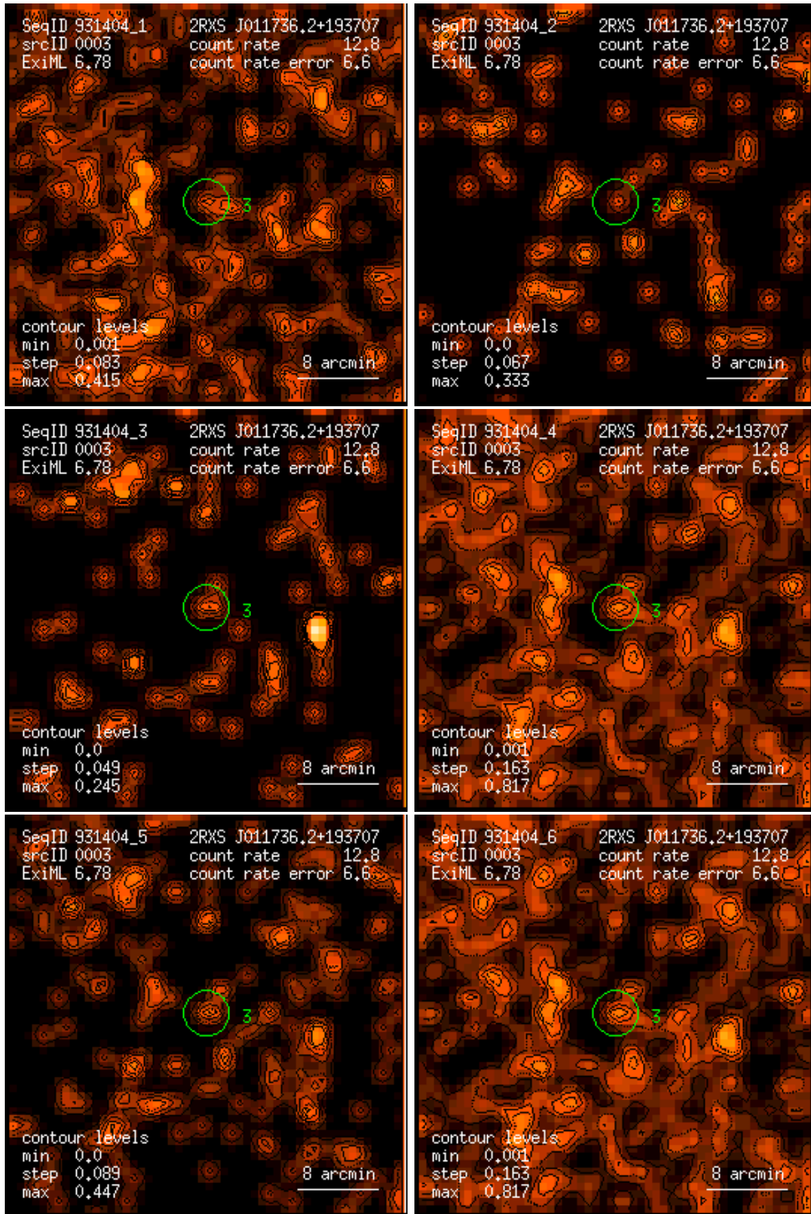
Figure 3: RASS 931404: detection 0003: band rate images, Gaussian filter: (1) PSPC channels 11 – 41, (2) 52 – 90, (3) 91 – 201, (4) 11 – 235, (5) 52 – 201, (6) 11 – 201. Broad band rates in counts/ks. Band rate contour levels in counts/ks/arcmin 2 .
