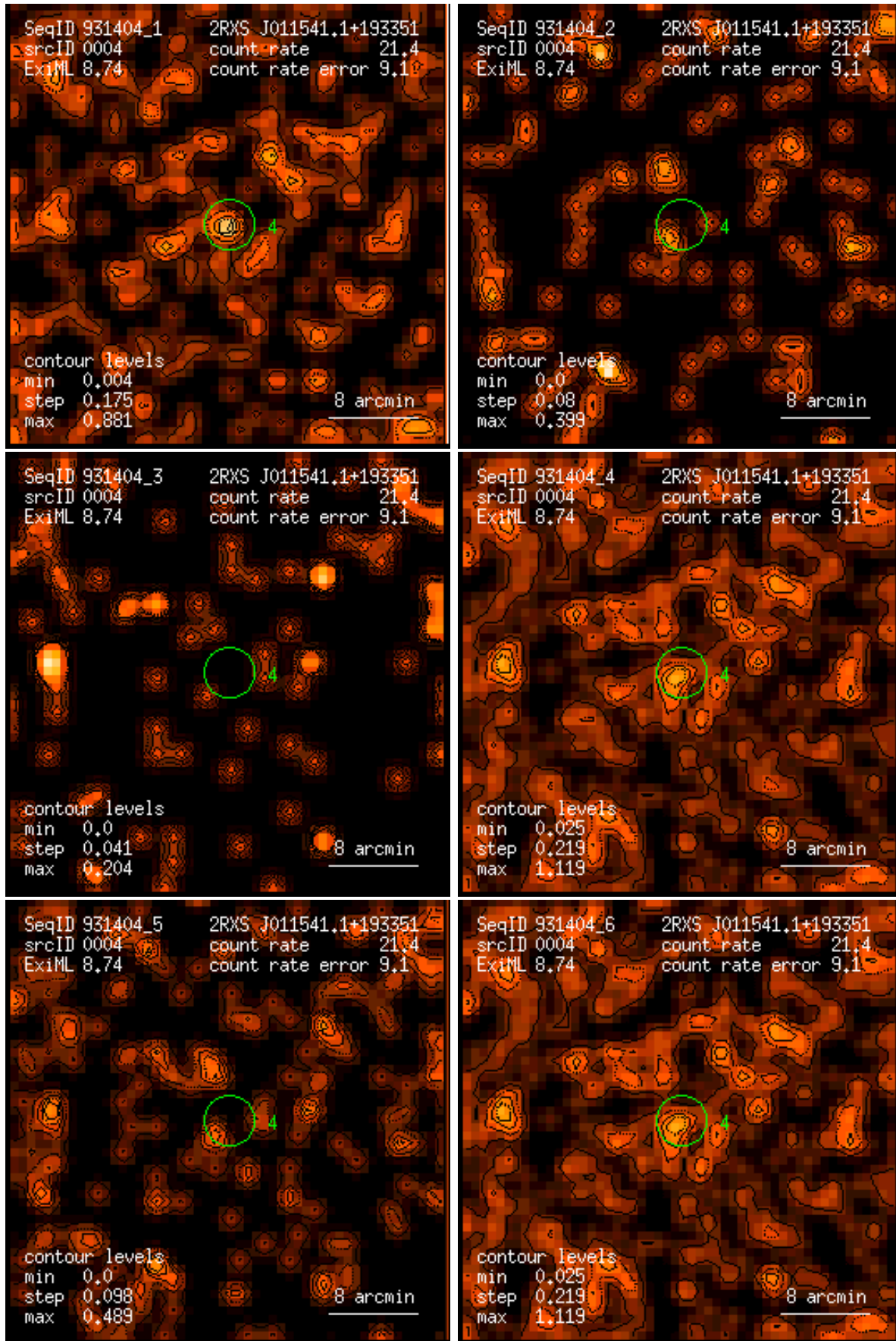
Figure 4: RASS 931404: detection 0004: band rate images, Gaussian filter: (1) PSPC channels 11 – 41, (2) 52 – 90, (3) 91 – 201, (4) 11 – 235, (5) 52 – 201, (6) 11 – 201. Broad band rates in counts/ks. Band rate contour levels in counts/ks/arcmin 2 .
