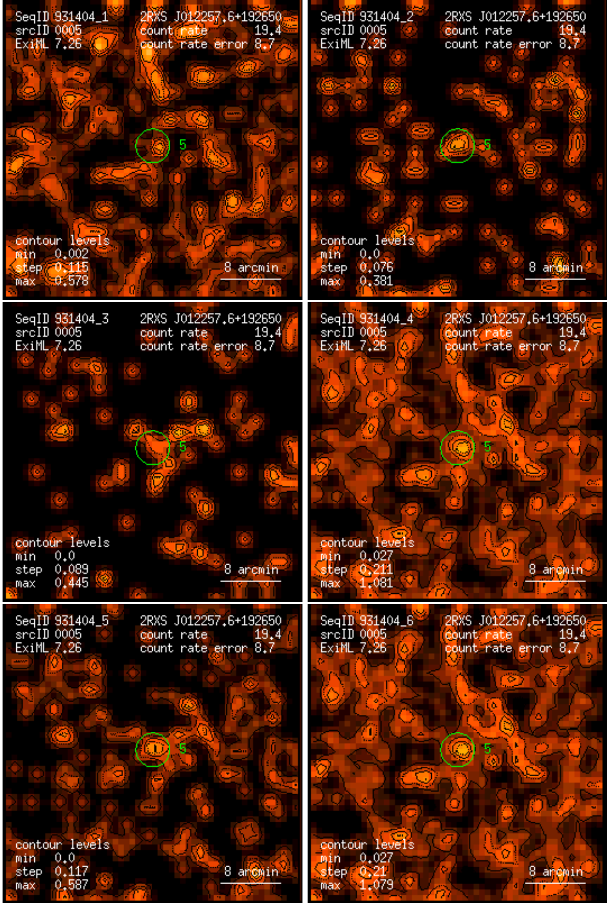
Figure 5: RASS 931404: detection 0005: band rate images, Gaussian filter: (1) PSPC channels 11 – 41, (2) 52 – 90, (3) 91 – 201, (4) 11 – 235, (5) 52 – 201, (6) 11 – 201. Broad band rates in counts/ks. Band rate contour levels in counts/ks/arcmin 2 .
