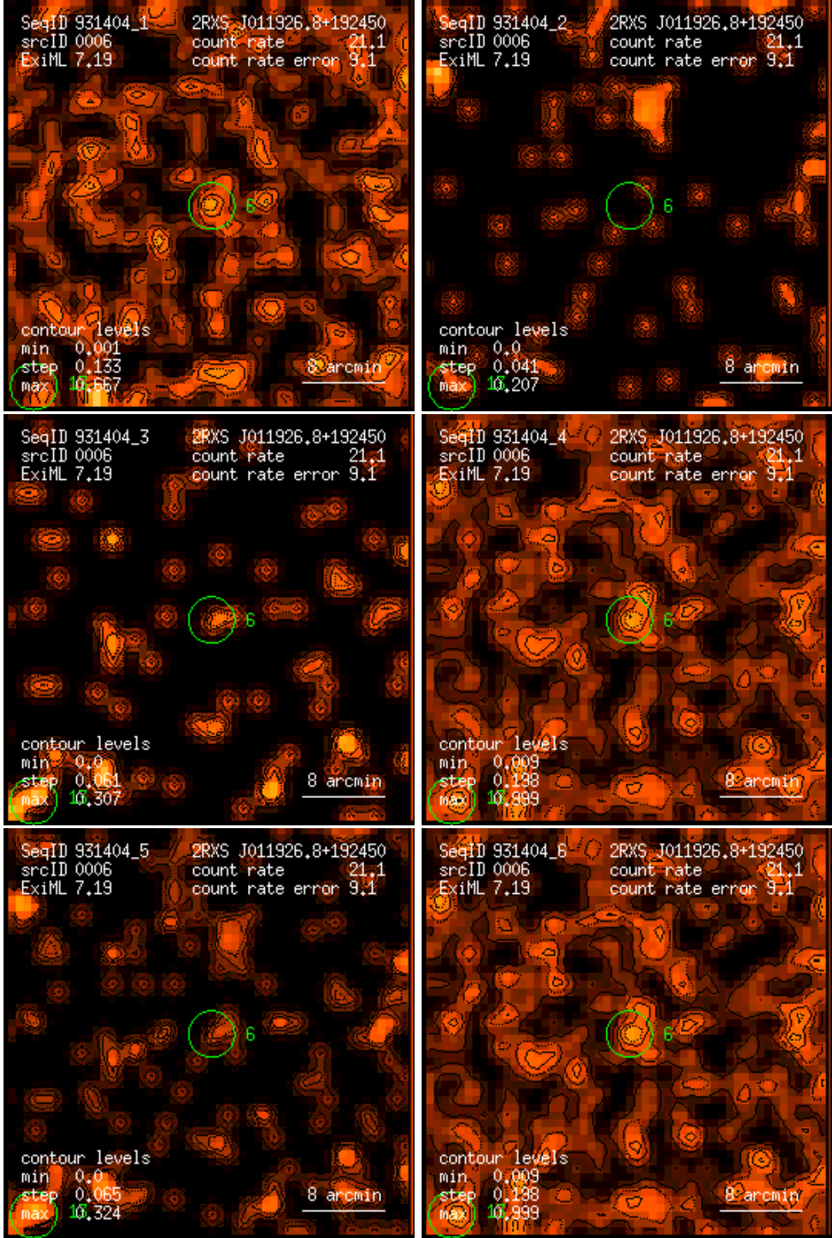
Figure 6: RASS 931404: detection 0006: band rate images, Gaussian filter: (1) PSPC channels 11 – 41, (2) 52 – 90, (3) 91 – 201, (4) 11 – 235, (5) 52 – 201, (6) 11 – 201. Broad band rates in counts/ks. Band rate contour levels in counts/ks/arcmin 2 .
