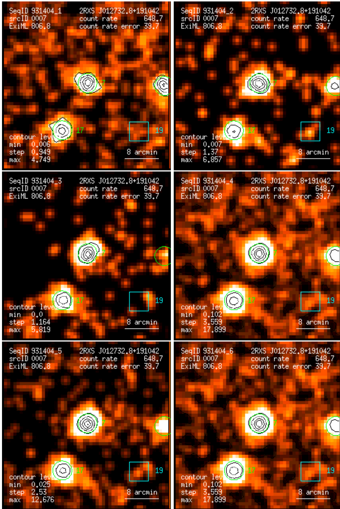
Figure 7: RASS 931404: detection 0007: band rate images, Gaussian filter: (1) PSPC channels 11 – 41, (2) 52 – 90, (3) 91 – 201, (4) 11 – 235, (5) 52 – 201, (6) 11 – 201. Broad band rates in counts/ks. Band rate contour levels in counts/ks/arcmin 2 .
