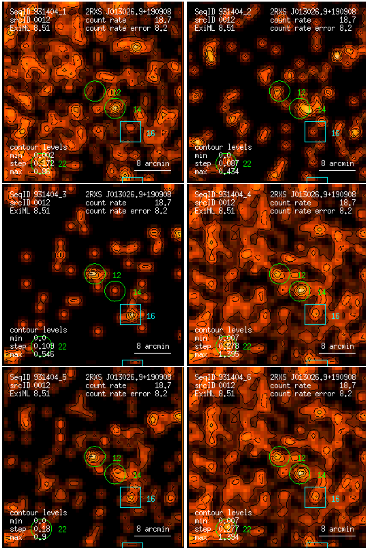
Figure 12: RASS 931404: detection 0012: band rate images, Gaussian filter: (1) PSPC channels 11 – 41, (2) 52 – 90, (3) 91 – 201, (4) 11 – 235, (5) 52 – 201, (6) 11 – 201. Broad band rates in counts/ks. Band rate contour levels in counts/ks/arcmin 2 .
