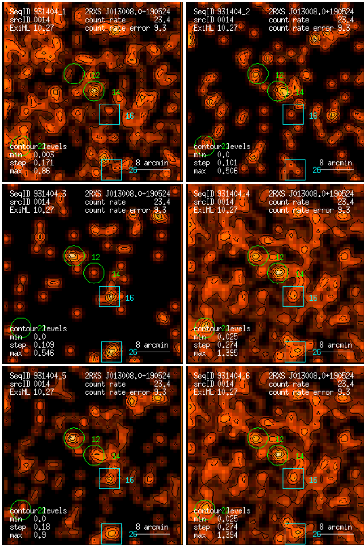
Figure 14: RASS 931404: detection 0014: band rate images, Gaussian filter: (1) PSPC channels 11 – 41, (2) 52 – 90, (3) 91 – 201, (4) 11 – 235, (5) 52 – 201, (6) 11 – 201. Broad band rates in counts/ks. Band rate contour levels in counts/ks/arcmin 2 .
